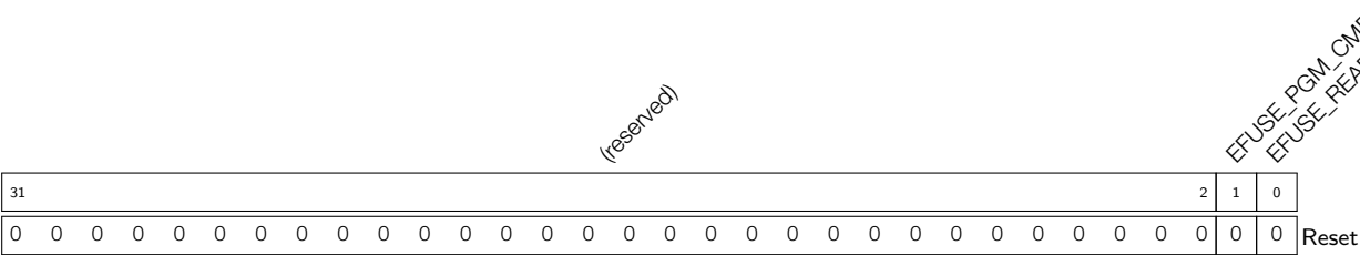
Register 20.23: EFUSE_CMD_REG (0x104)
