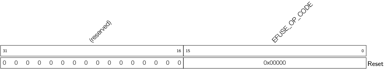
Register 20.22: EFUSE_CONF_REG (0x0fc)
