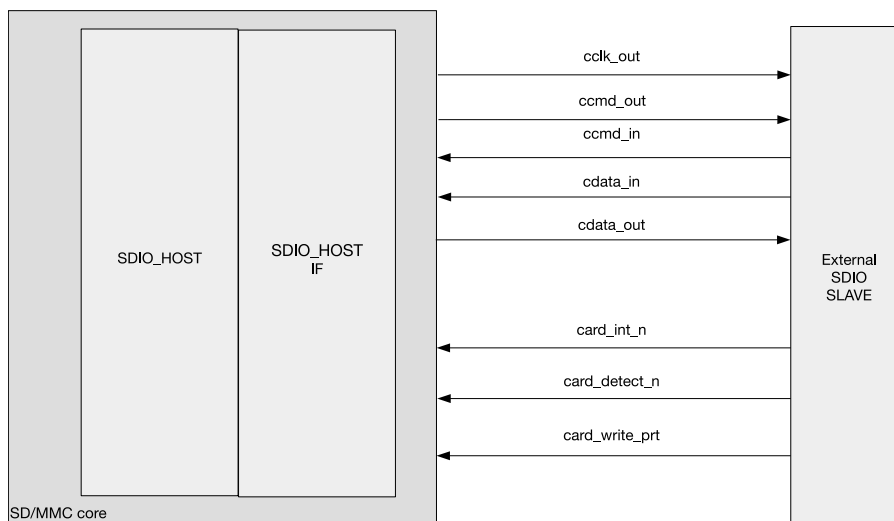
Figure 31: SD/MMC Controller External Interface Signals
