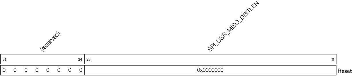
Register 7.12: SPI_MISO_DLEN_REG (0x2C)
