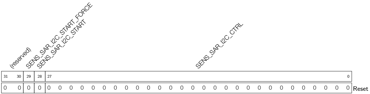
Register 29.7: SENS_SAR_I2C_CTRL_REG (0x0050)
