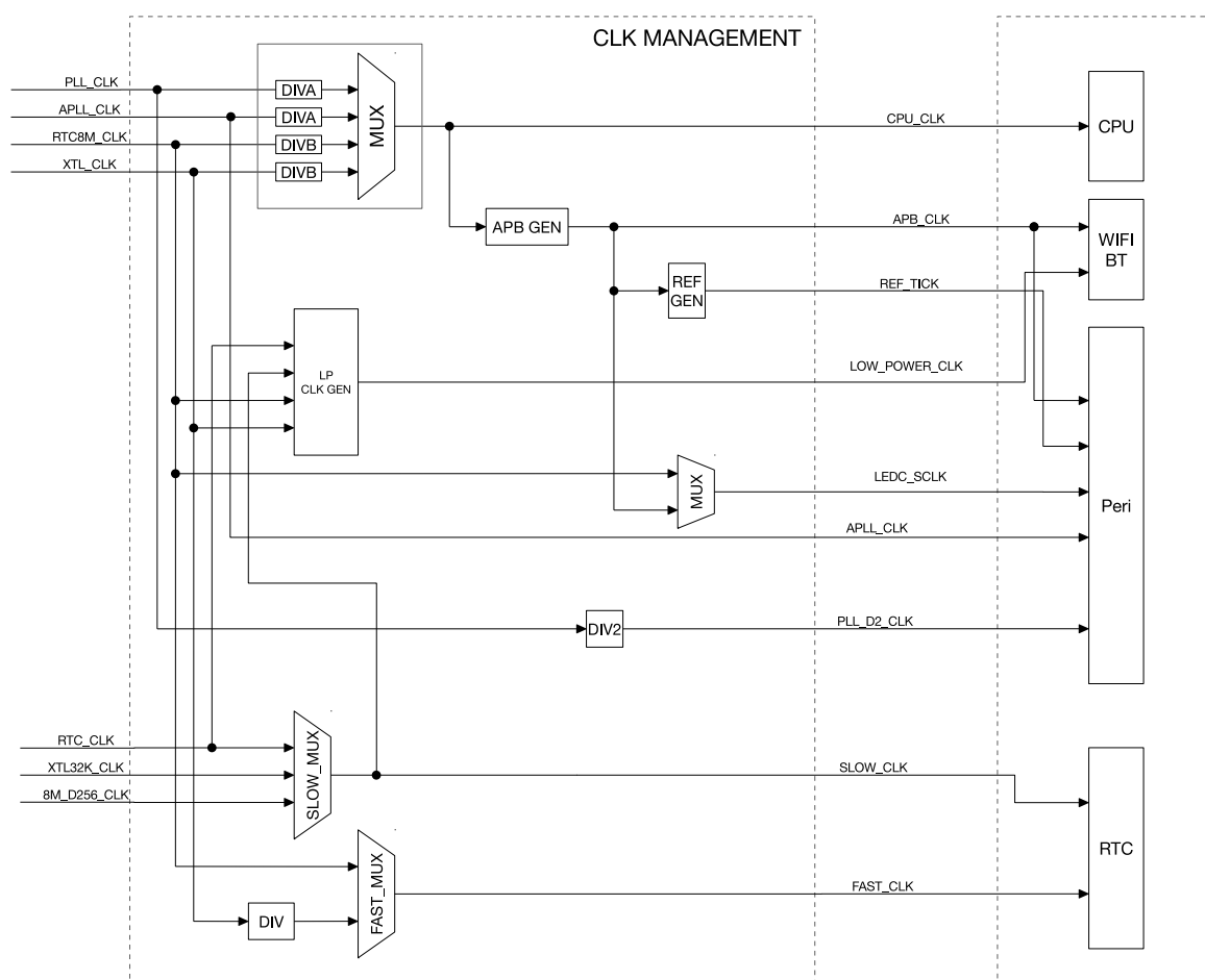
Figure 6: System Clock
