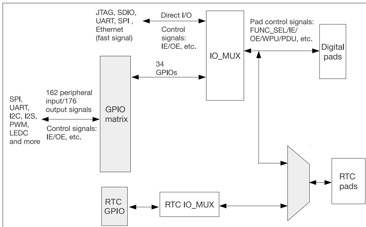
Figure 7: IO_MUX, RTC IO_MUX and GPIO Matrix Overview
