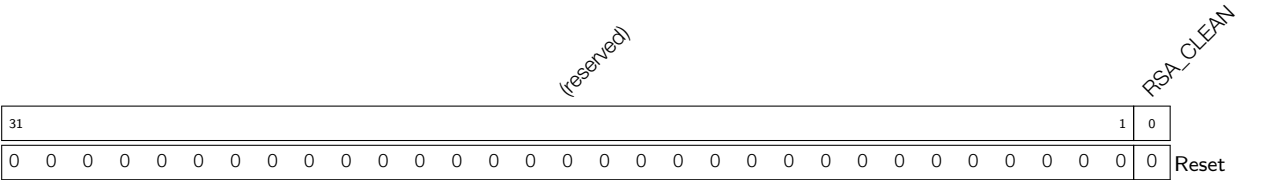
Register 23.7: RSA_CLEAN_REG (0x818)
