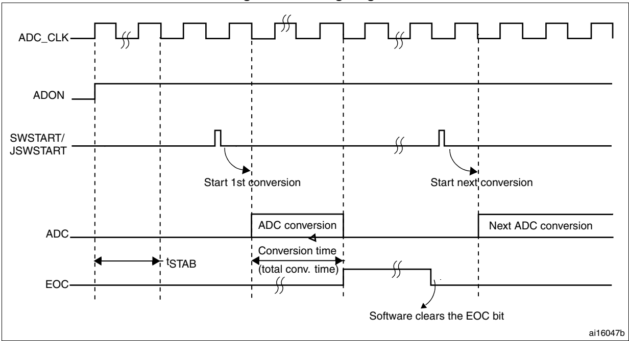
Figure 60. Timing diagram
