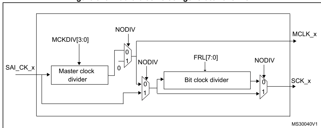
Figure 345. Audio block clock generator overview
