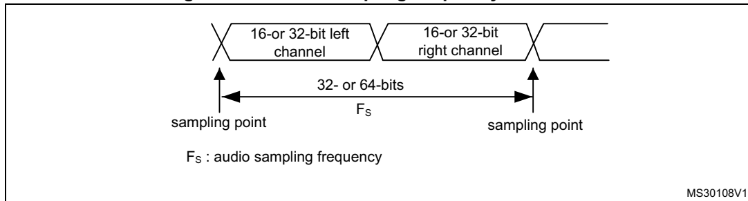
Figure 337. Audio sampling frequency definition
