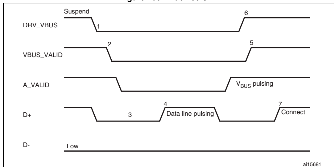
Figure 403. A-device SRP
