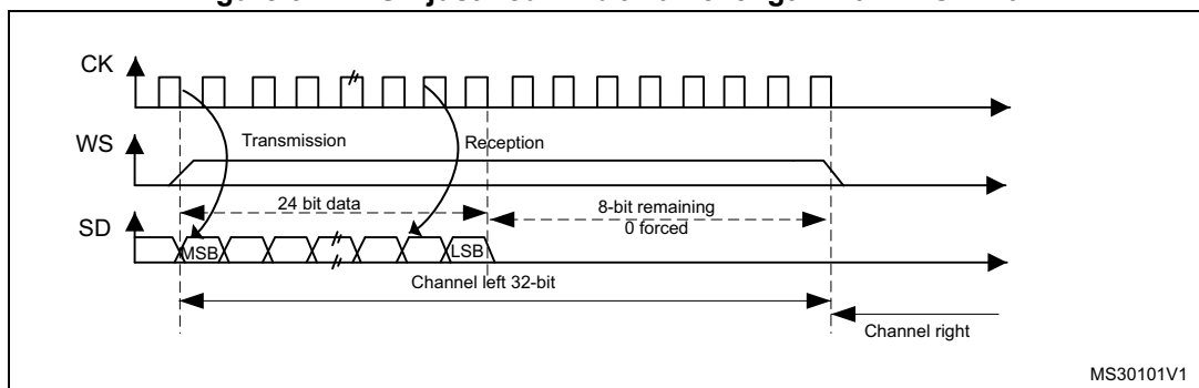
Figure 327. MSB justified 24-bit frame length with CPOL = 0
