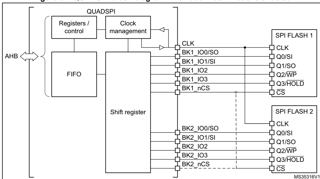
Figure 52. QUADSPI block diagram when dual-flash mode is enabled
