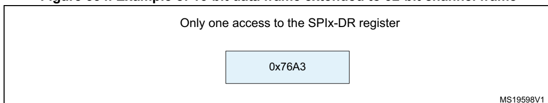
Figure 334. Example of 16-bit data frame extended to 32-bit channel frame
