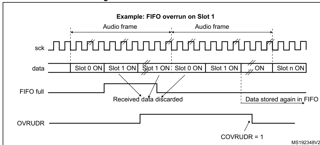
Figure 350. Overrun detection error
