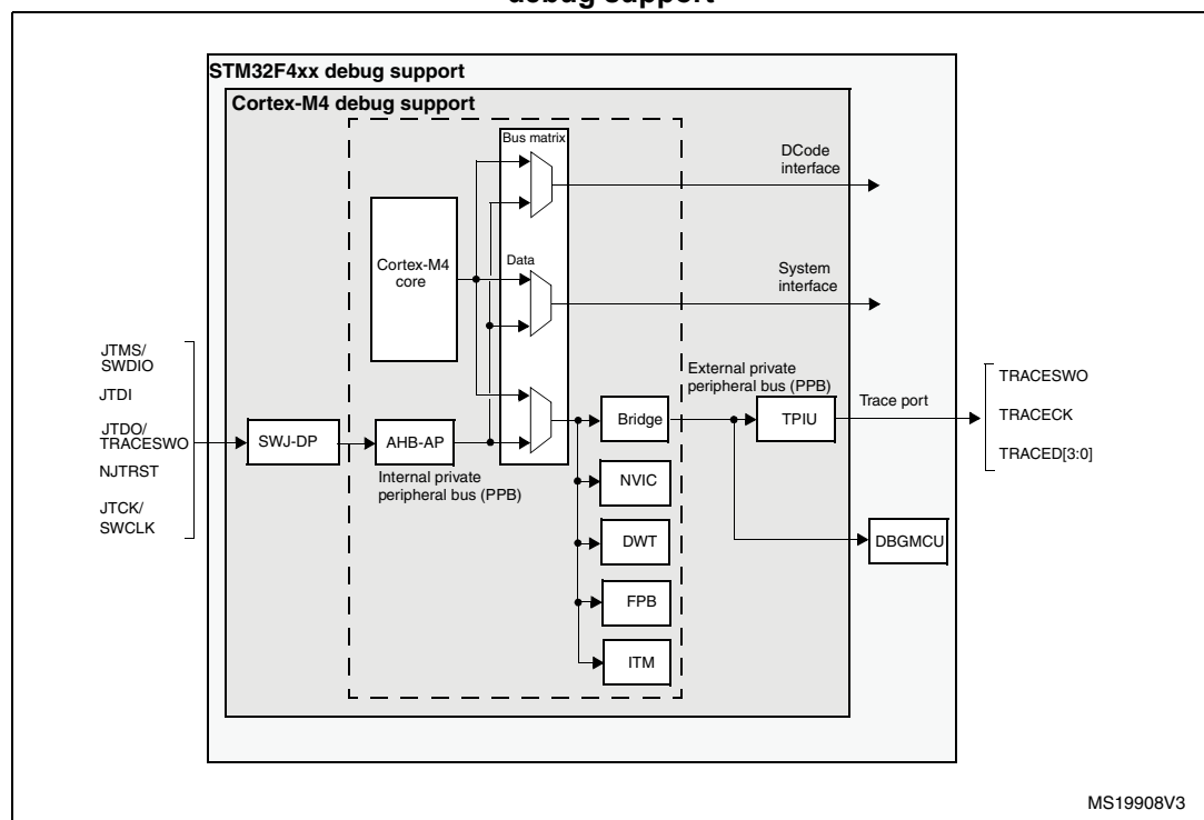
Figure 407. Block diagram of STM32 MCU and Cortex ® -M4 with FPU-level debug support
