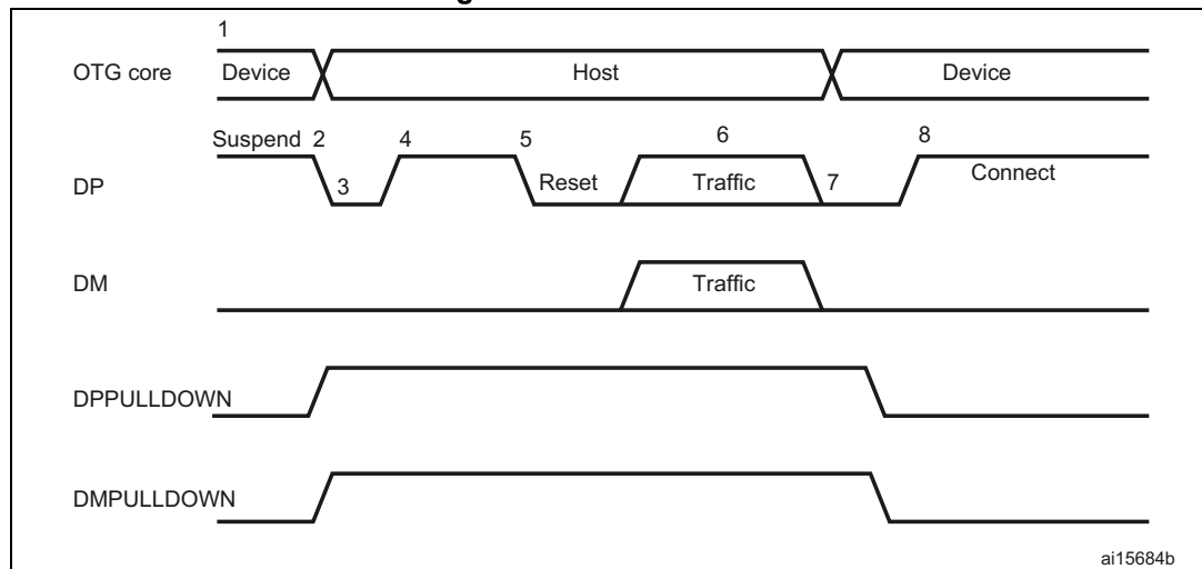
Figure 406. B-device HNP
