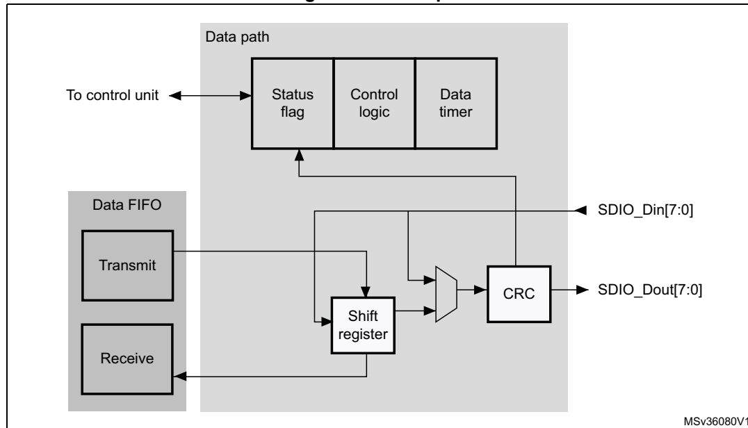
Figure 364. Data path
