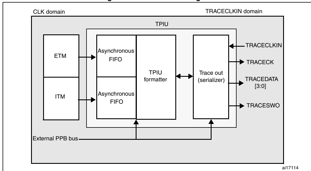
Figure 410. TPIU block diagram
