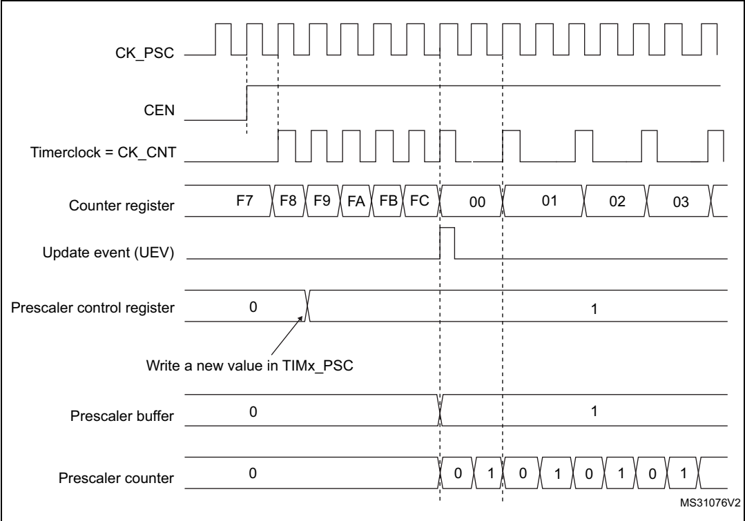
Figure 88. Counter timing diagram with prescaler division change from 1 to 2
