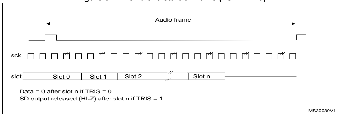
Figure 342. FS role is start of frame (FSDEF = 0)
