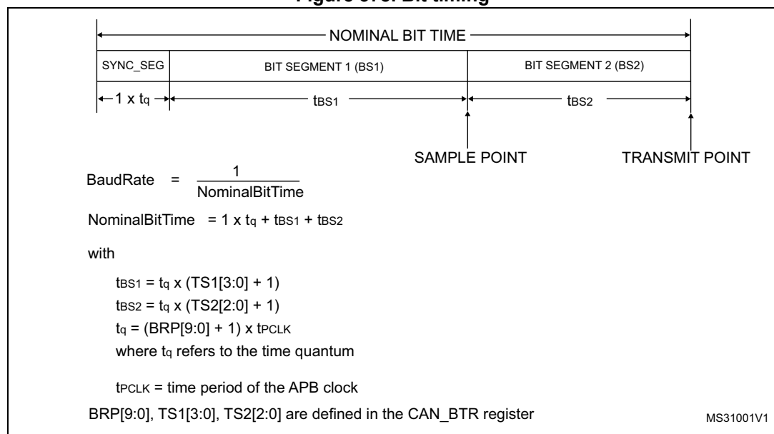
Figure 378. Bit timing
