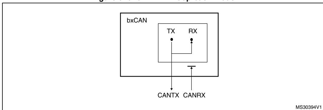
Figure 370. bxCAN in loop back mode
