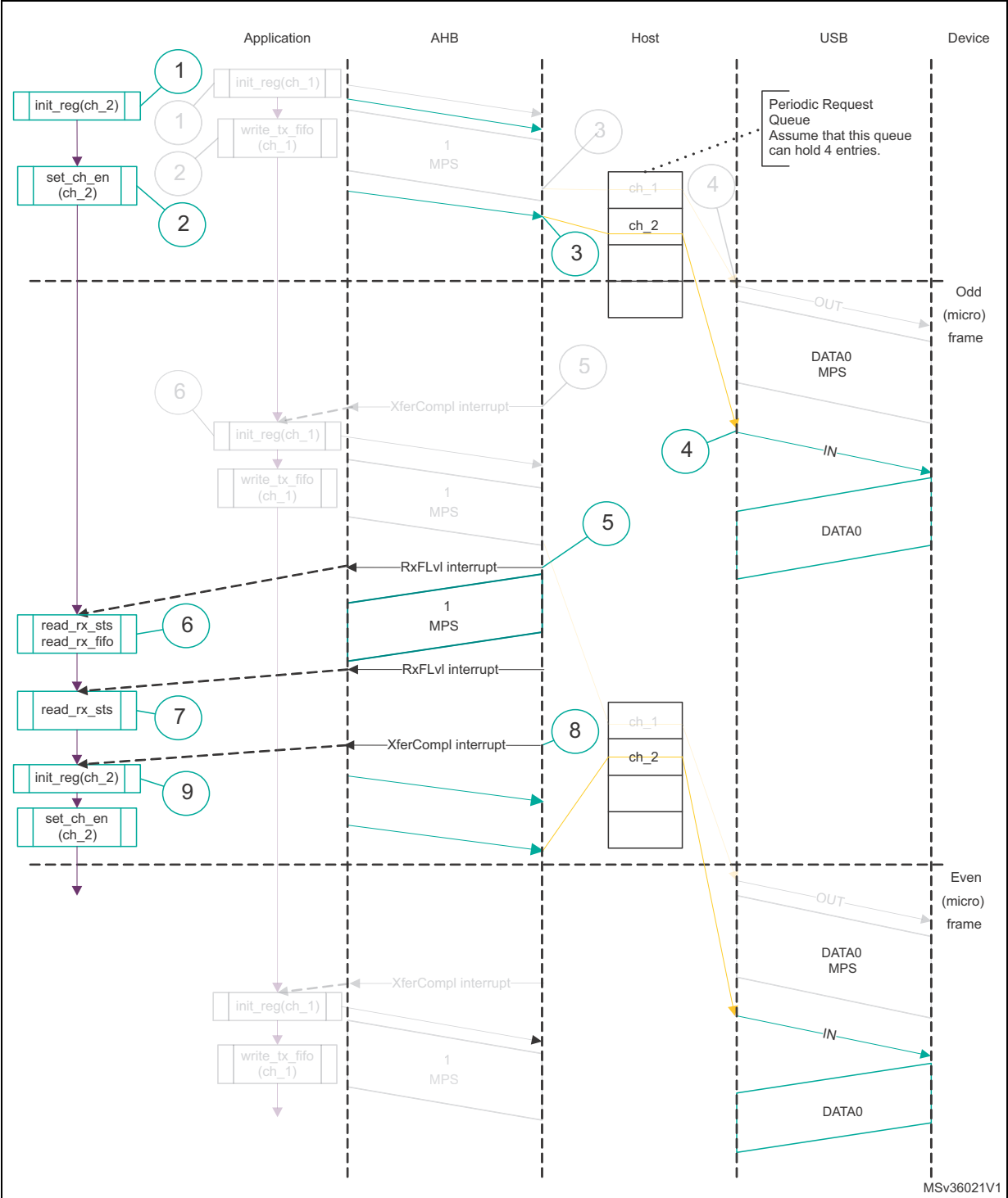
Figure 398. Isochronous IN transactions
