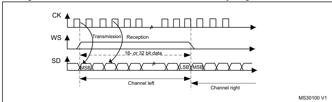
Figure 326. MSB Justified 16-bit or 32-bit full-accuracy length with CPOL = 0
