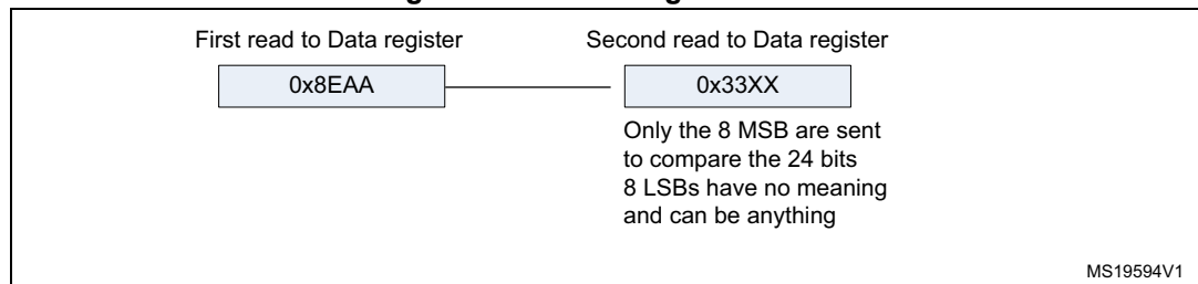
Figure 323. Receiving 0x8EAA33
