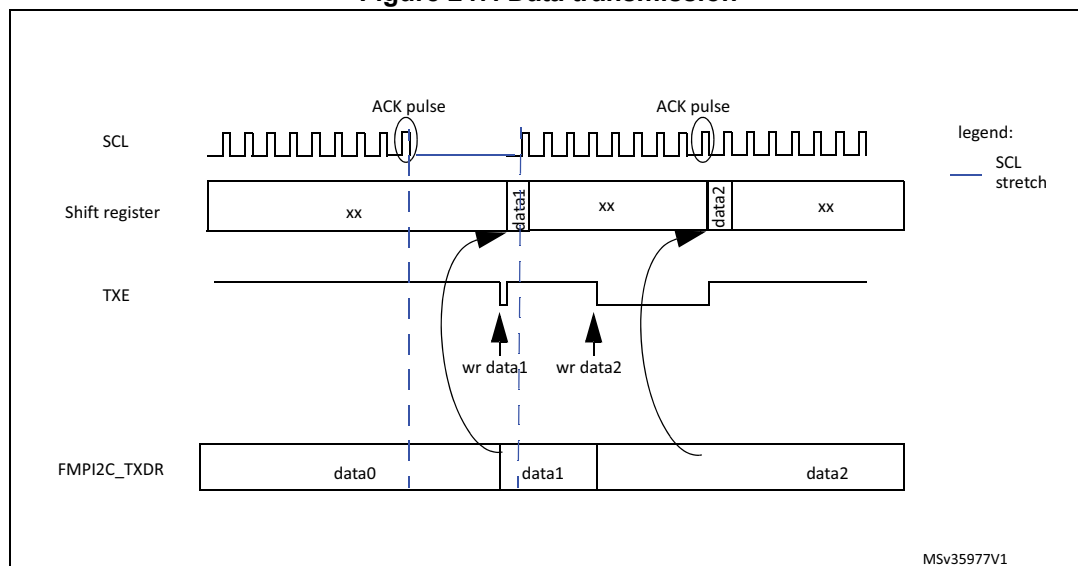
Figure 247. Data transmission
