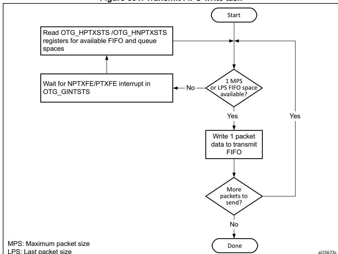
Figure 391. Transmit FIFO write task
