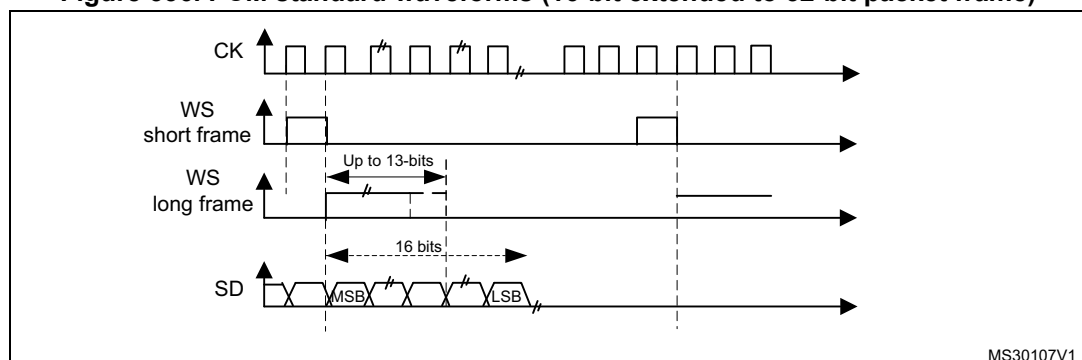
Figure 336. PCM standard waveforms (16-bit extended to 32-bit packet frame)
