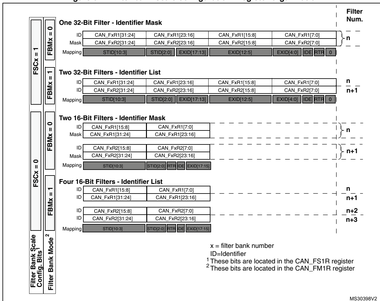
Figure 374. Filter bank scale configuration - register organization
