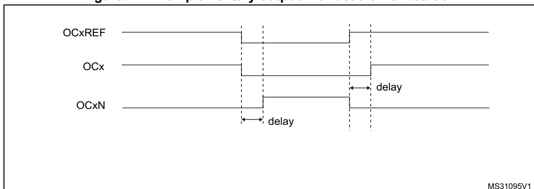
Figure 121. Complementary output with dead-time insertion.
