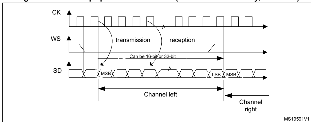
Figure 320. I 2 S Philips protocol waveforms (16/32-bit full accuracy, CPOL = 0)
