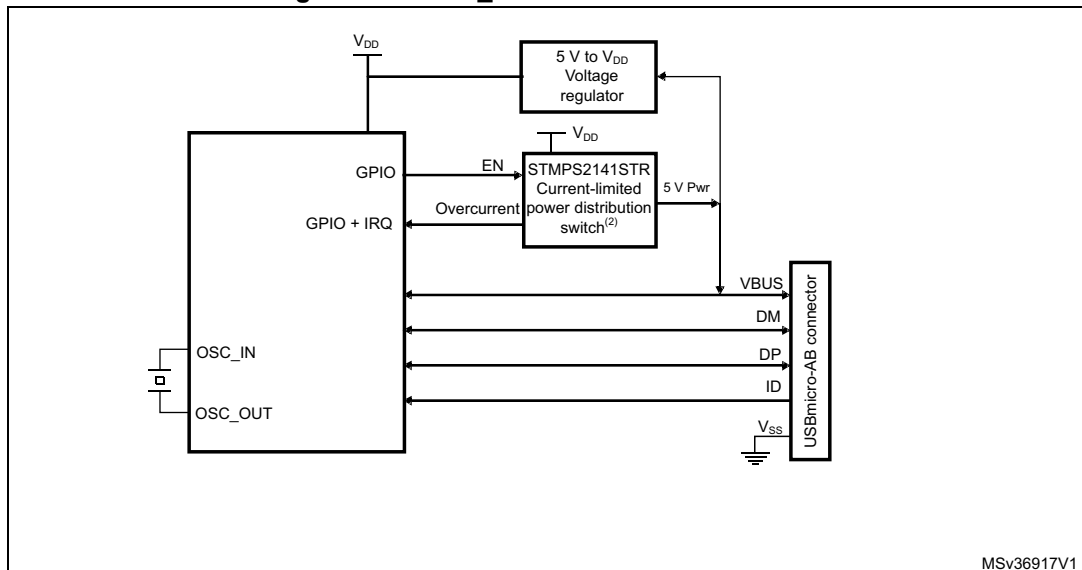
Figure 383. OTG_FS A-B device connection
