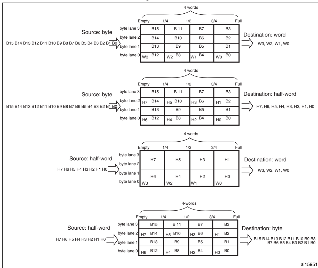
Figure 28. FIFO structure
