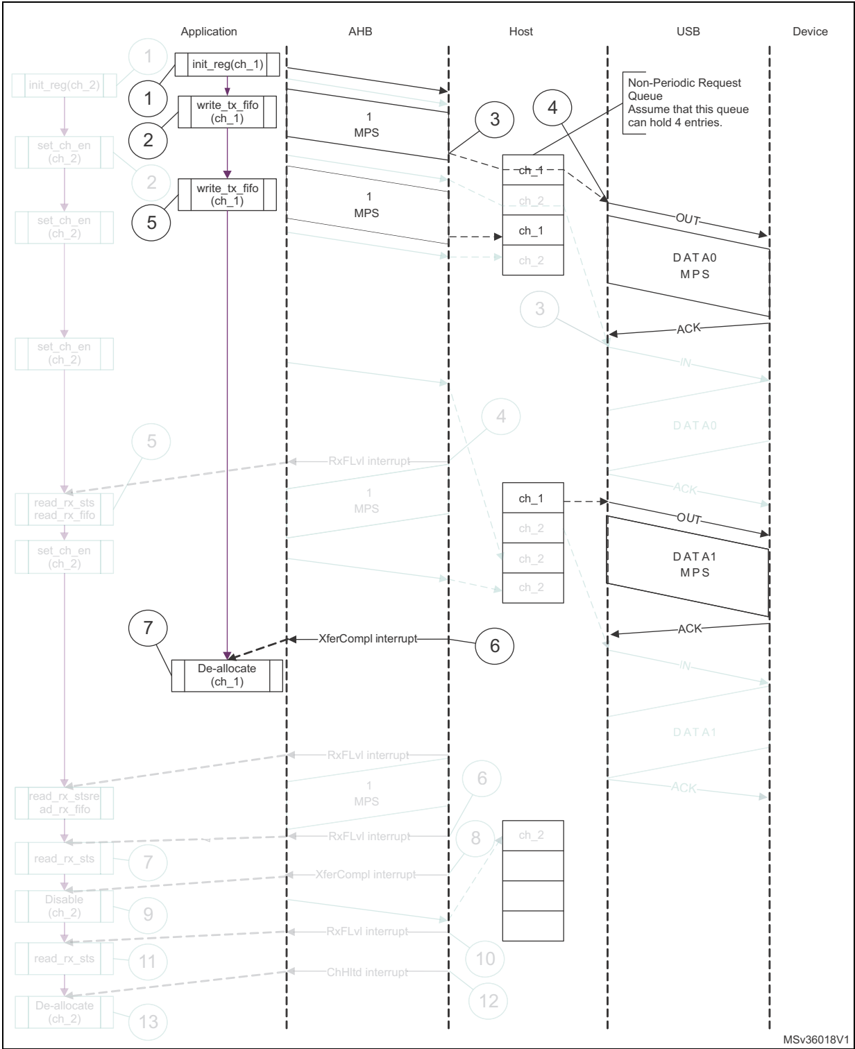
Figure 393. Normal bulk/control OUT/SETUP
