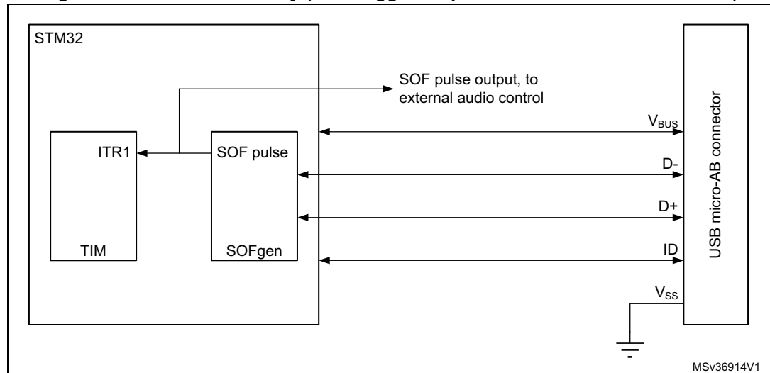
Figure 386. SOF connectivity (SOF trigger output to TIM and ITR1 connection)
