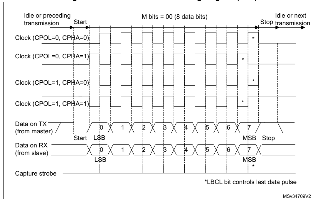
Figure 292. USART data clock timing diagram (M=0)
