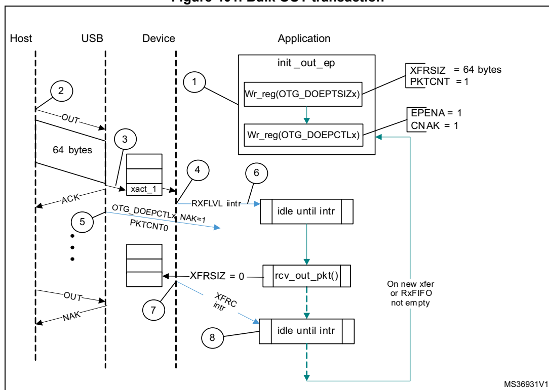
Figure 401. Bulk OUT transaction
