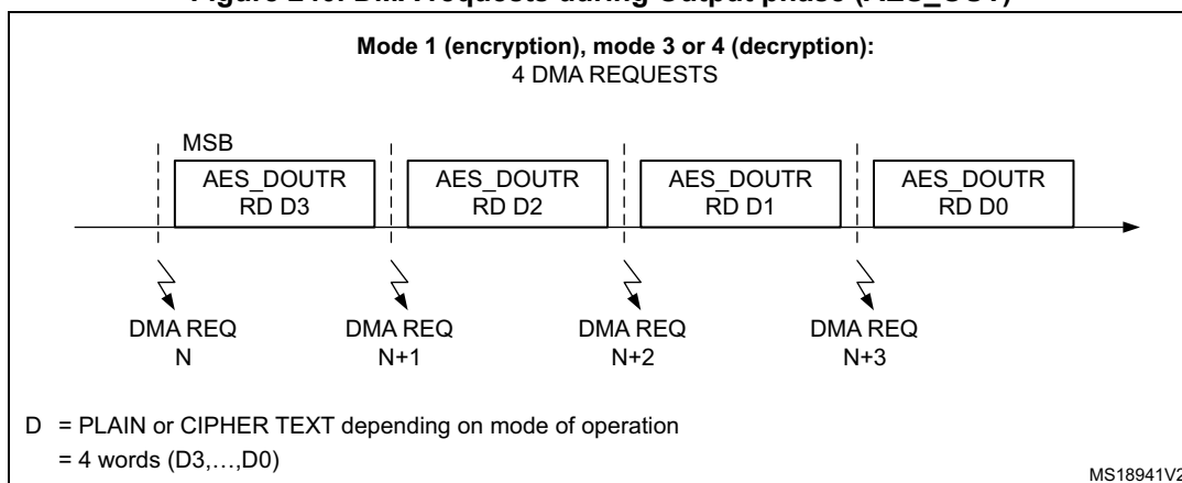
Figure 240. DMA requests during Output phase (AES_OUT)
