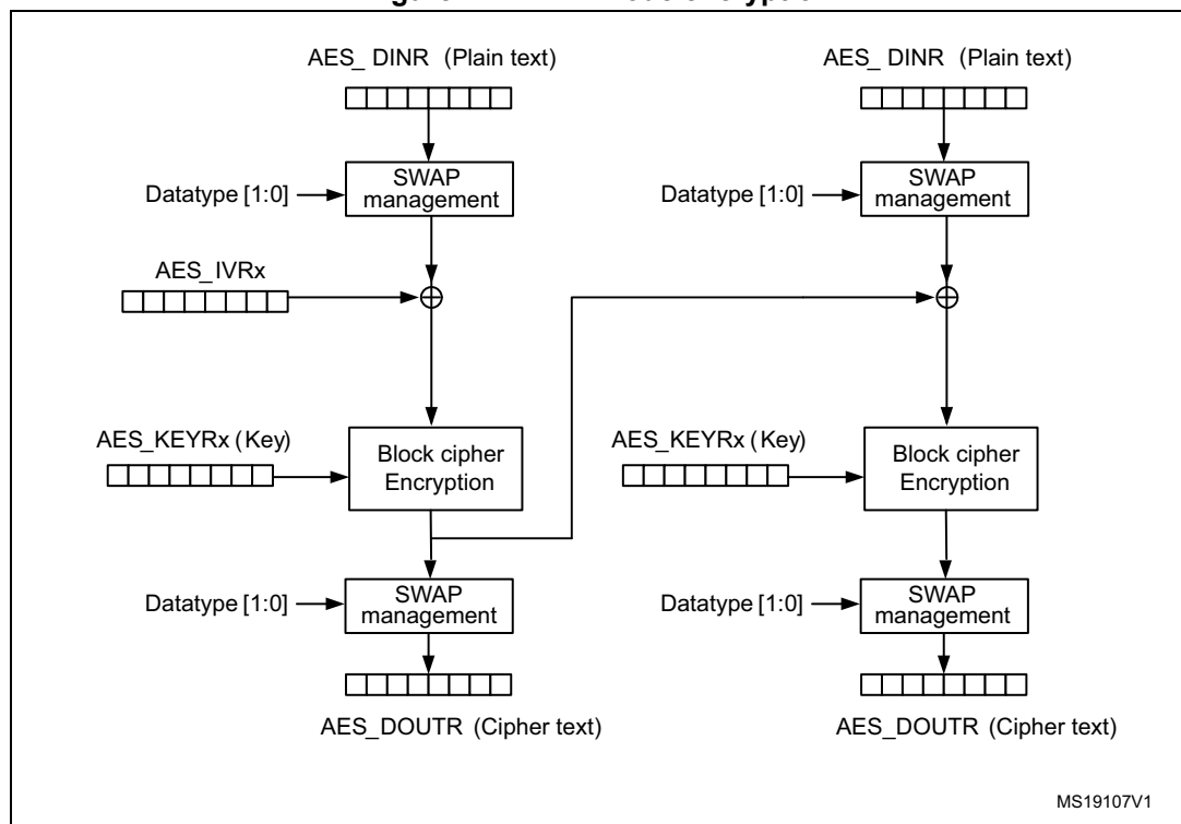
Figure 227. CBC mode encryption
