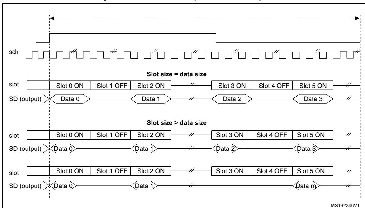
Figure 349. Tristate on output data line in a protocol like I2S
