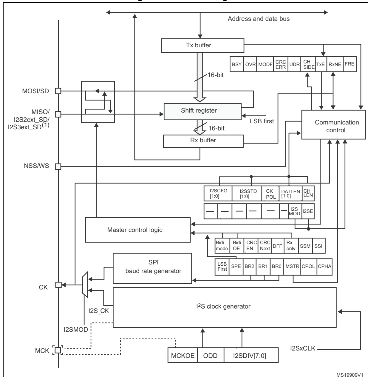
Figure 318. I 2 S block diagram
