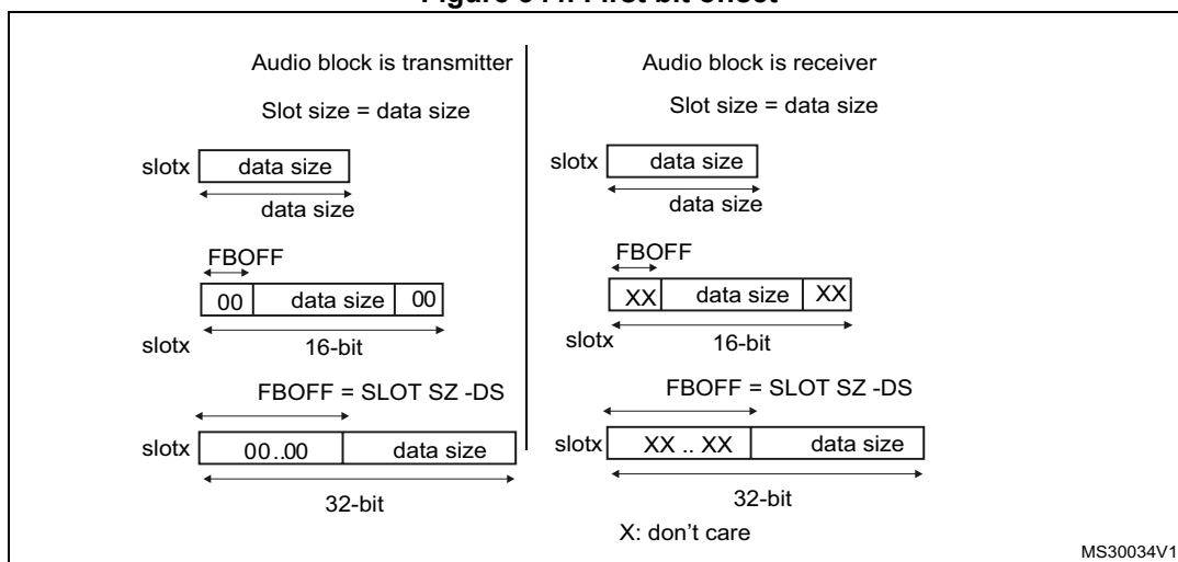
Figure 344. First bit offset
