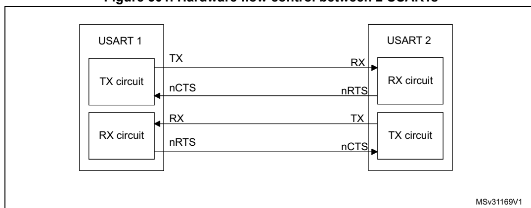
Figure 301. Hardware flow control between 2 USARTs
