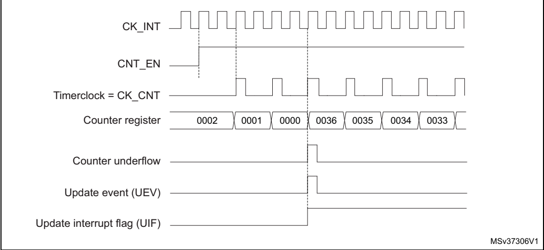
Figure 145. Counter timing diagram, internal clock divided by 2
