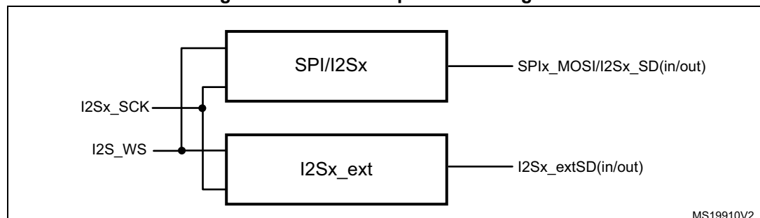
Figure 319. I2S full-duplex block diagram
