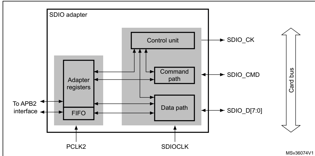
Figure 358. SDIO adapter
