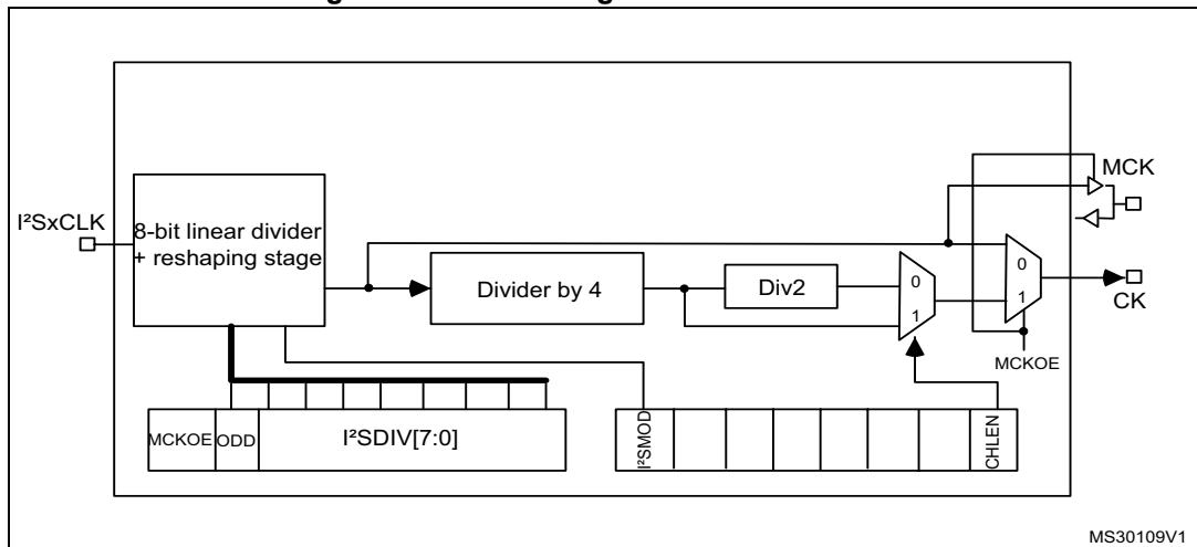
Figure 338. I 2 S clock generator architecture
