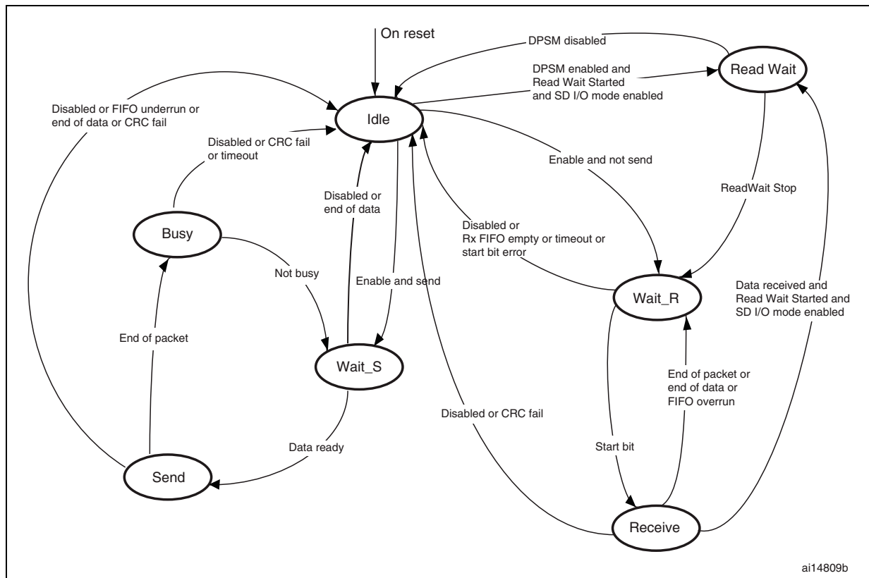
Figure 365. Data path state machine (DPSM)
