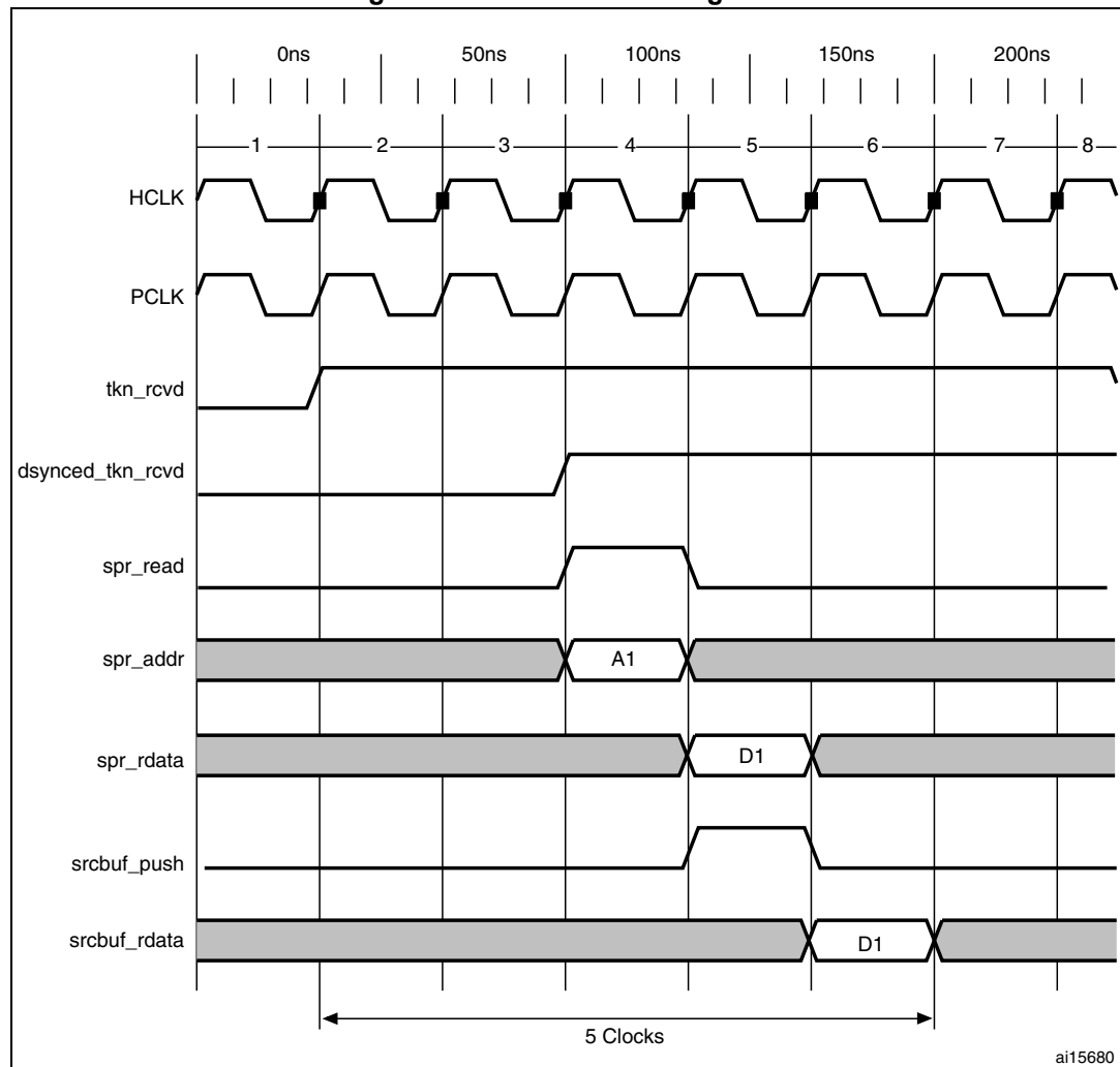
Figure 402. TRDT max timing case
