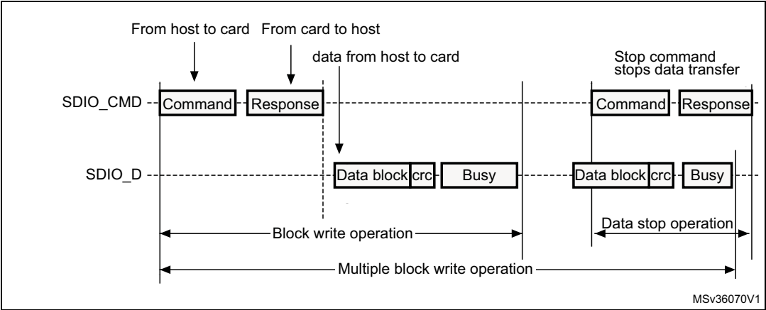
Figure 354. (Multiple) block write operation
