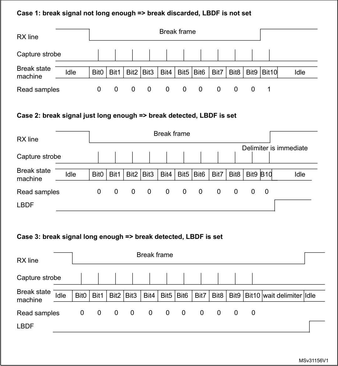
Figure 289. Break detection in LIN mode (11-bit break length - LBDL bit is set)
