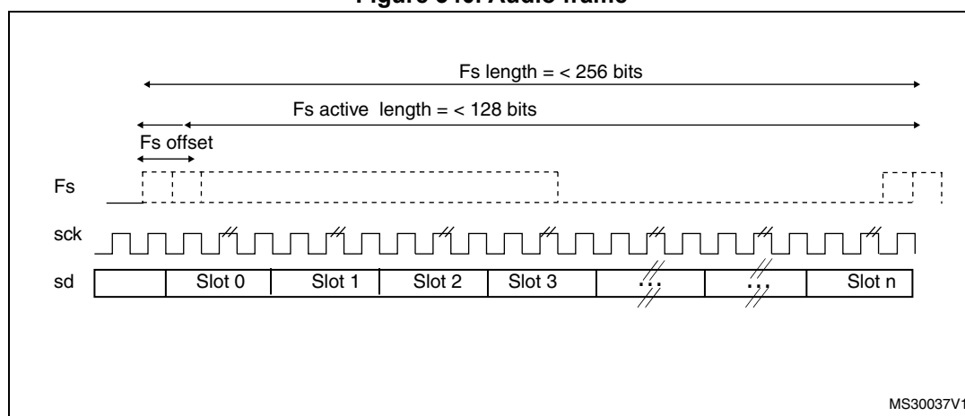
Figure 340. Audio frame
