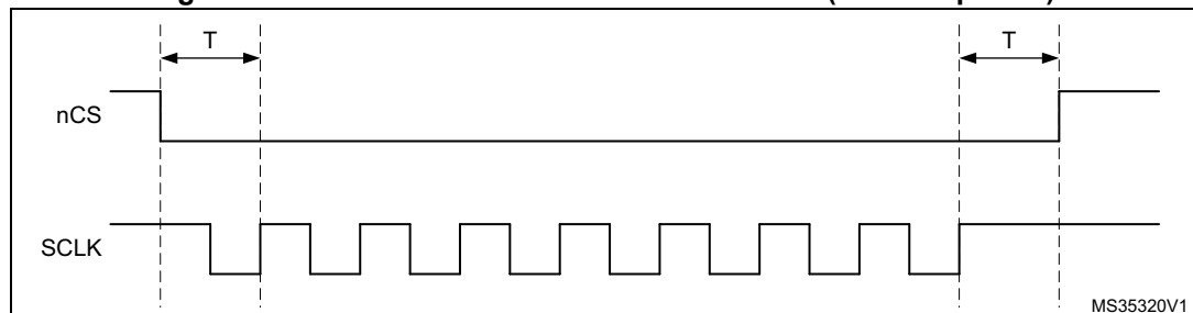
Figure 56. nCS when CKMODE = 1 in SDR mode (T = CLK period)
