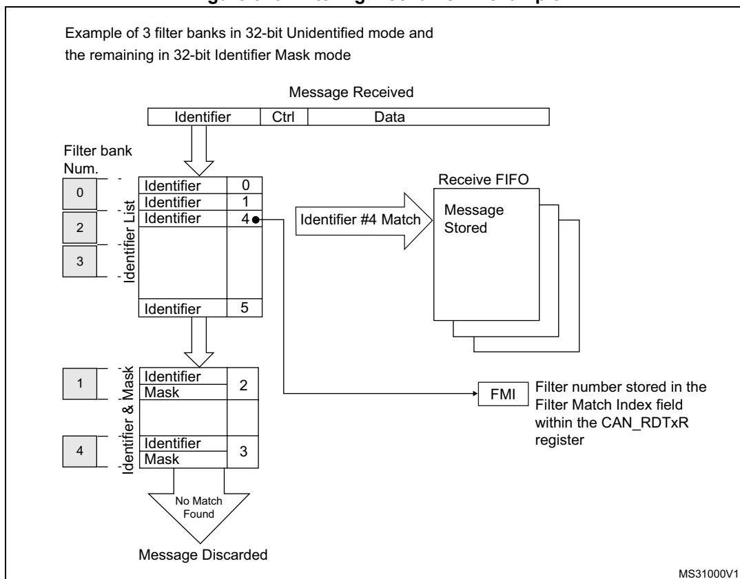
Figure 376. Filtering mechanism - example
