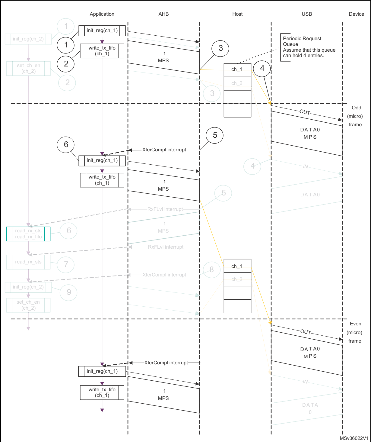
Figure 397. Isochronous OUT transactions
