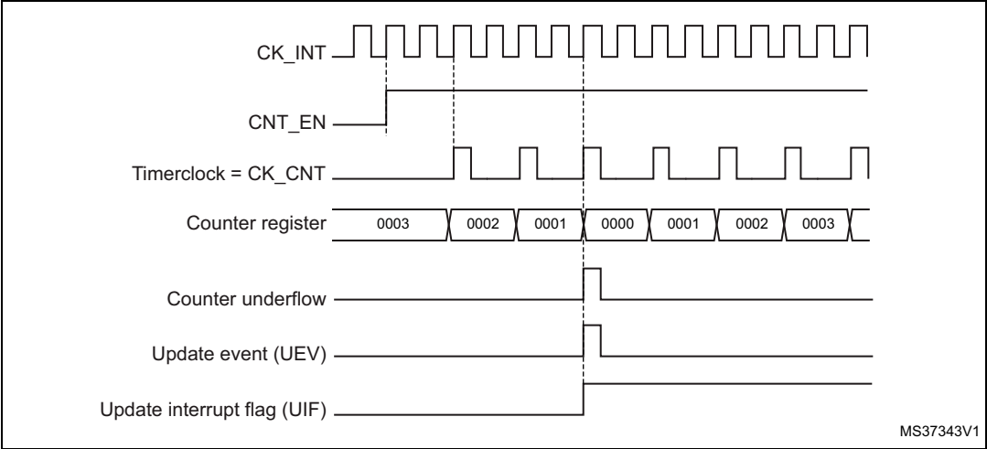
Figure 150. Counter timing diagram, internal clock divided by 2
