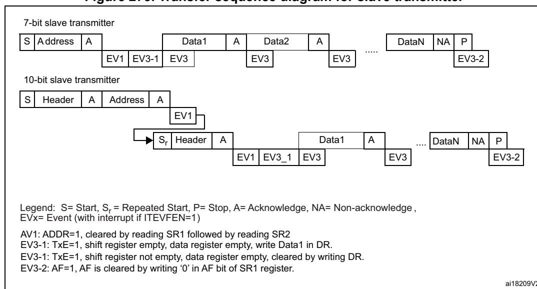
Figure 275. Transfer sequence diagram for slave transmitter
