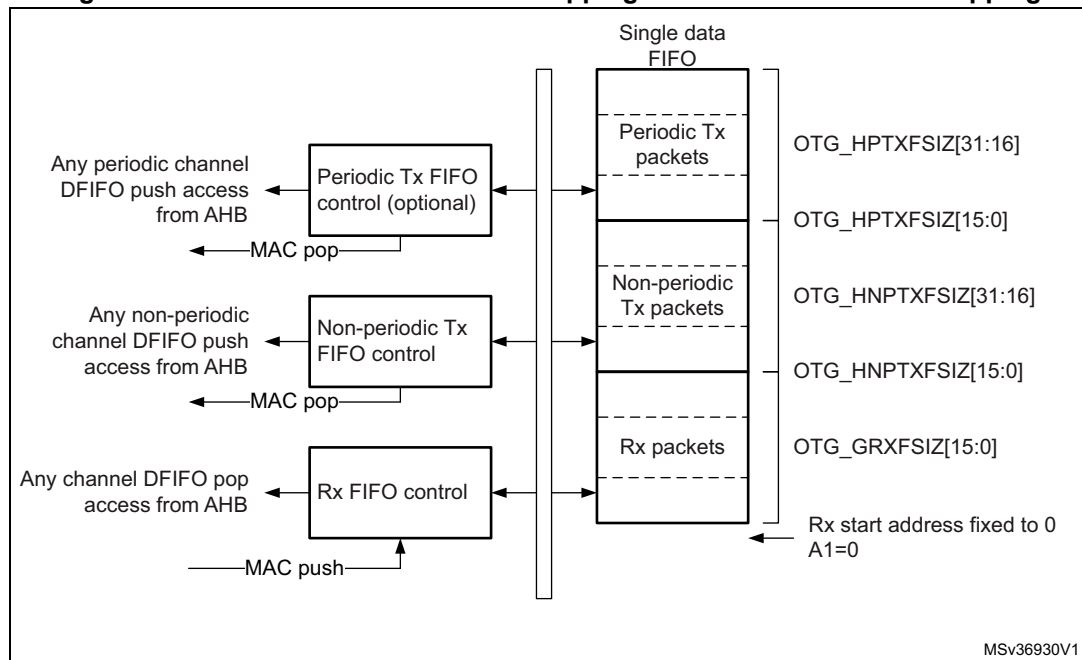
Figure 389. Host-mode FIFO address mapping and AHB FIFO access mapping
