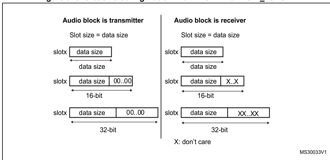
Figure 343. Slot size configuration with FBOFF = 0 in SAI_xSLOTR
