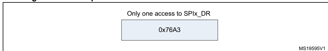
Figure 325. Example of 16-bit data frame extended to 32-bit channel frame
