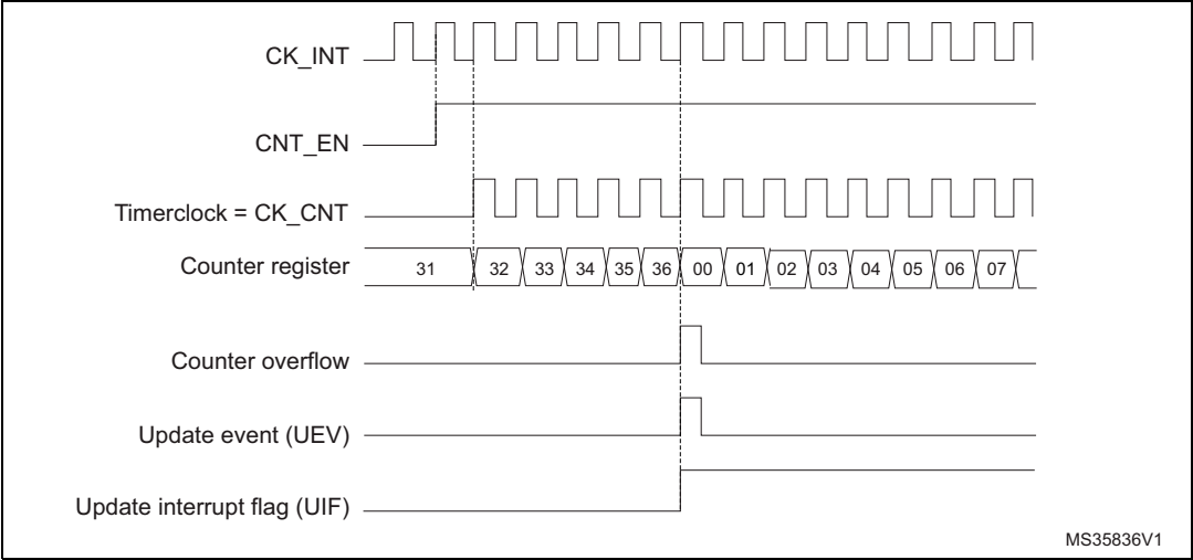
Figure 138. Counter timing diagram, internal clock divided by 1
