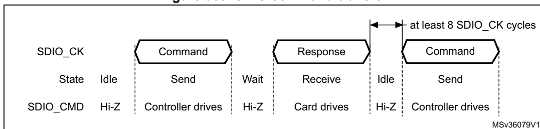
Figure 363. SDIO command transfer
