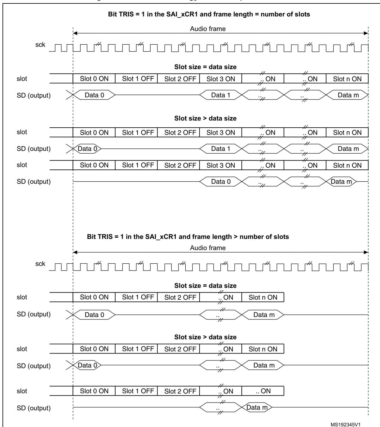
Figure 348. Tristate strategy on SD output line on an inactive slot
