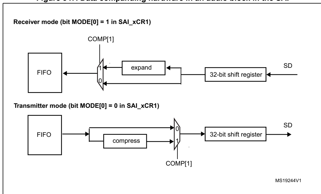
Figure 347. Data companding hardware in an audio block in the SAI
