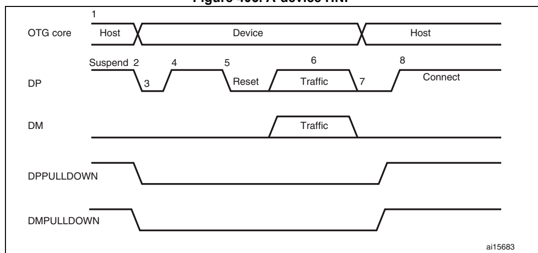
Figure 405. A-device HNP
