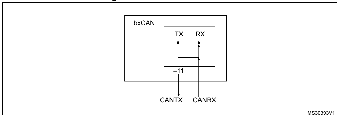
Figure 369. bxCAN in silent mode
