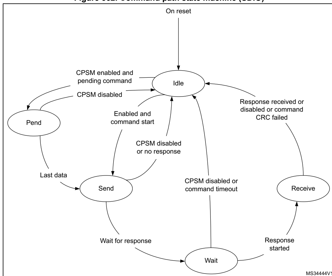
Figure 362. Command path state machine (SDIO)
