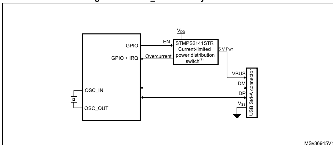
Figure 385. USB_FS host-only connection
