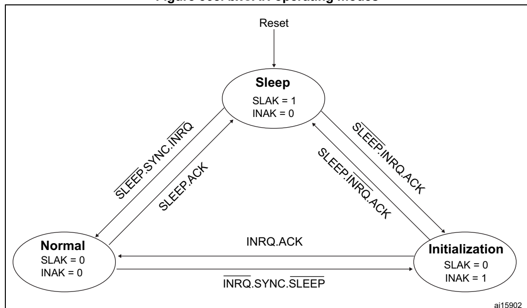
Figure 368. bxCAN operating modes
