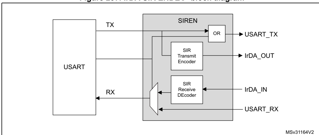
Figure 297. IrDA SIR ENDEC- block diagram
