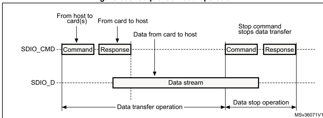
Figure 355. Sequential read operation
