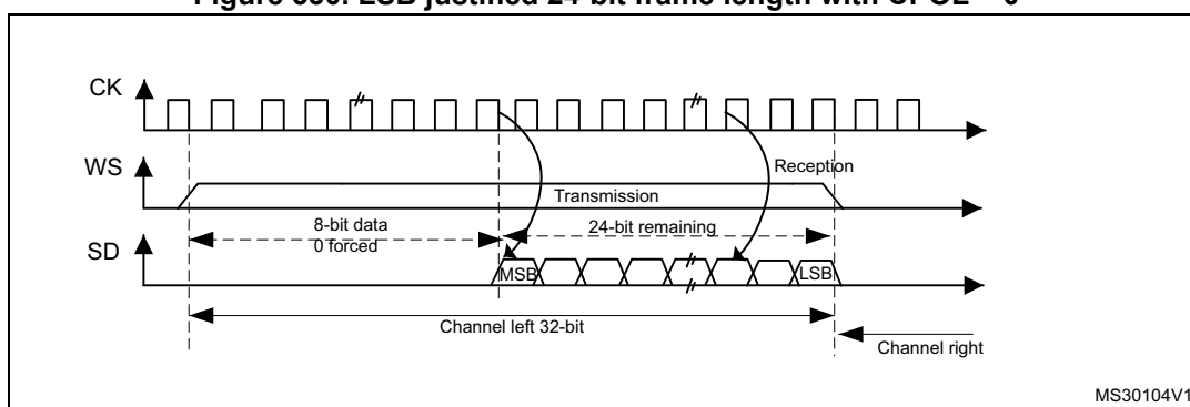
Figure 330. LSB justified 24-bit frame length with CPOL = 0
