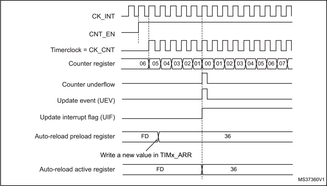
Figure 153. Counter timing diagram, Update event with ARPE=1 (counter underflow)
