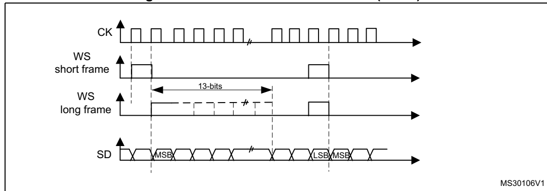
Figure 335. PCM standard waveforms (16-bit)
