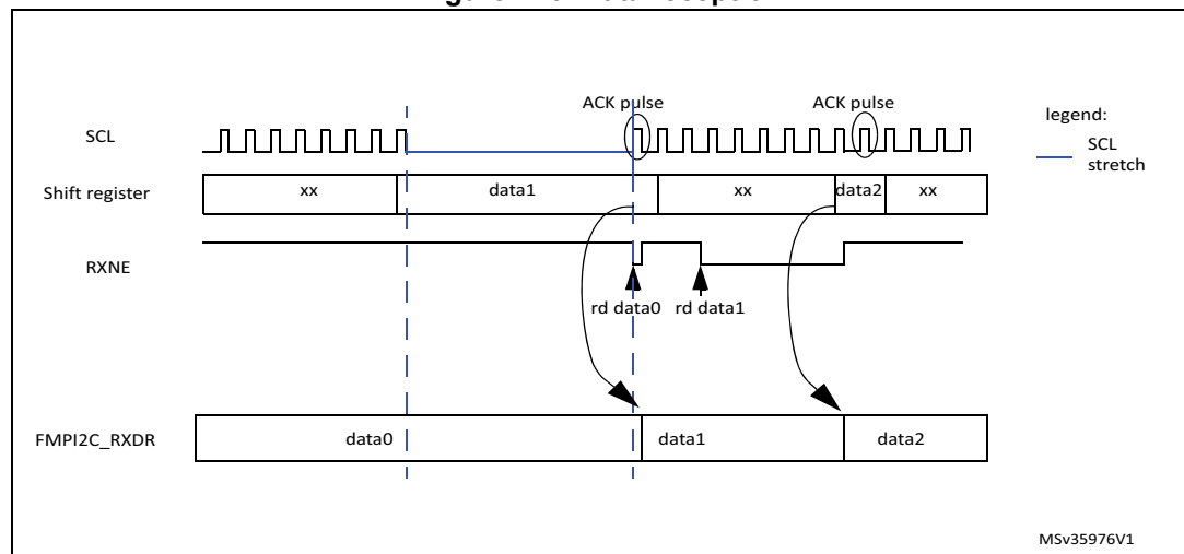
Figure 246. Data reception
