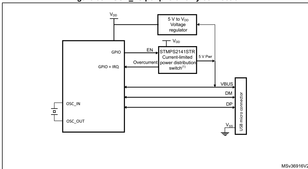
Figure 384. USB_FS peripheral-only connection
