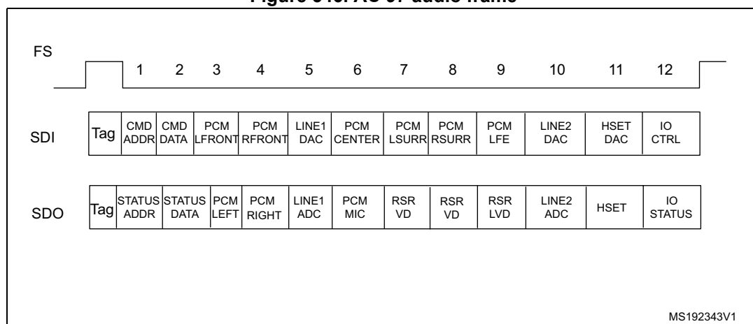
Figure 346. AC'97 audio frame
