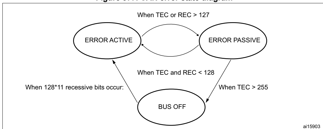
Figure 377. CAN error state diagram
