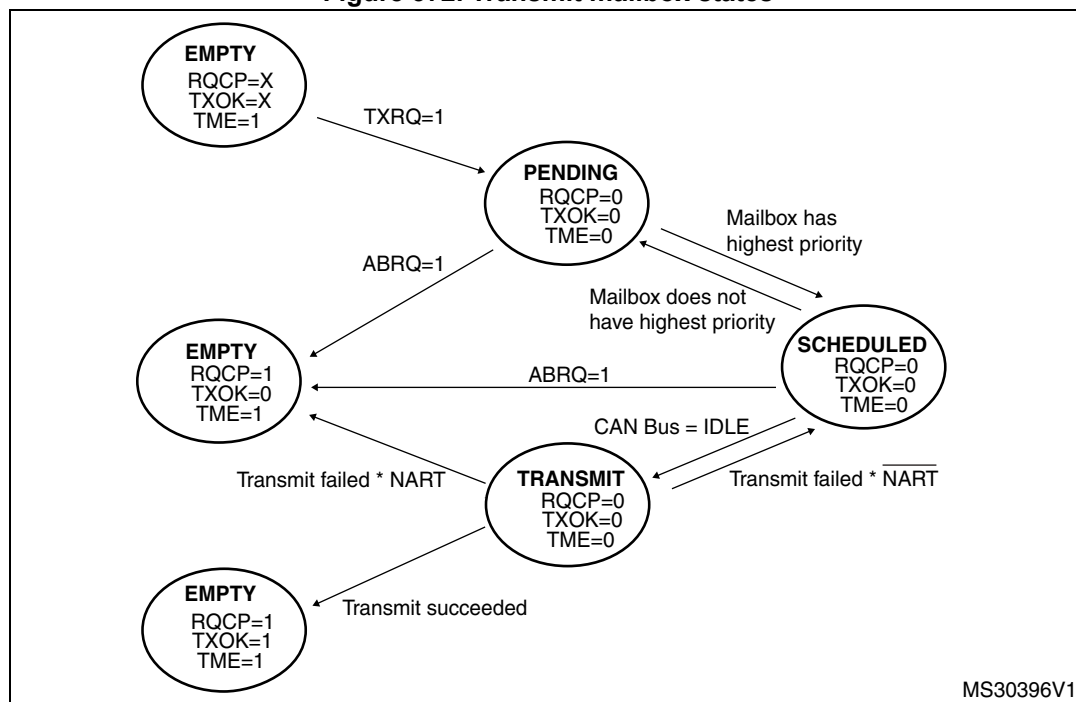
Figure 372. Transmit mailbox states
