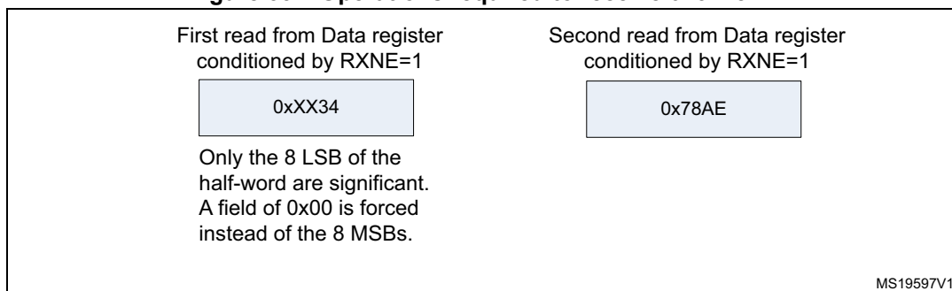
Figure 332. Operations required to receive 0x3478AE
