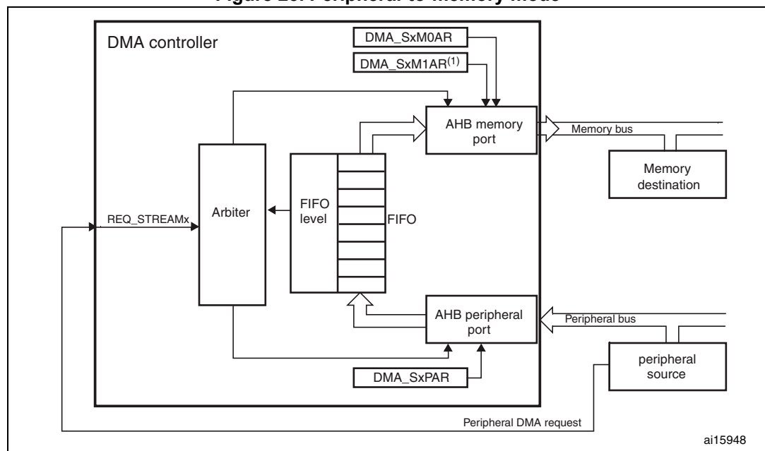
Figure 25. Peripheral-to-memory mode
