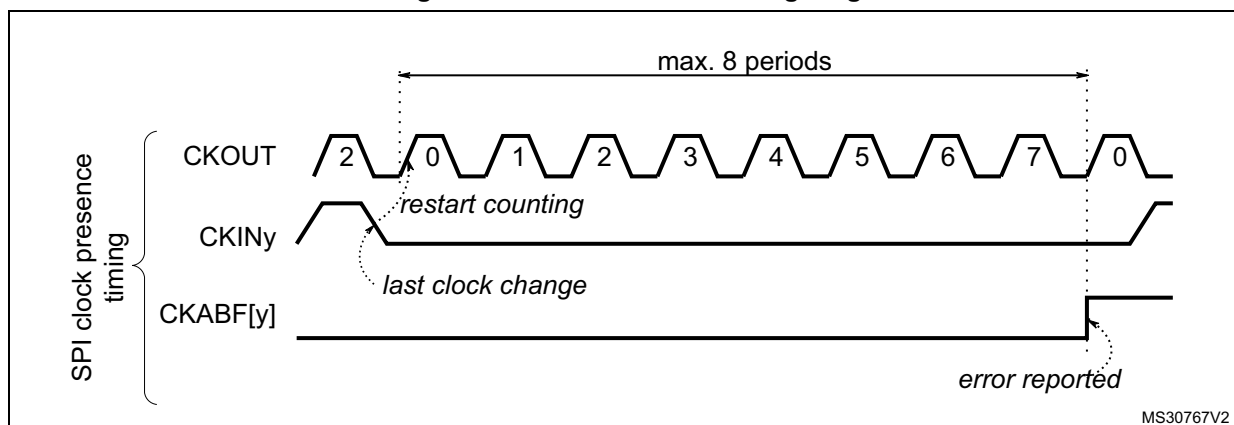
Figure 78. Clock absence timing diagram for SPI
