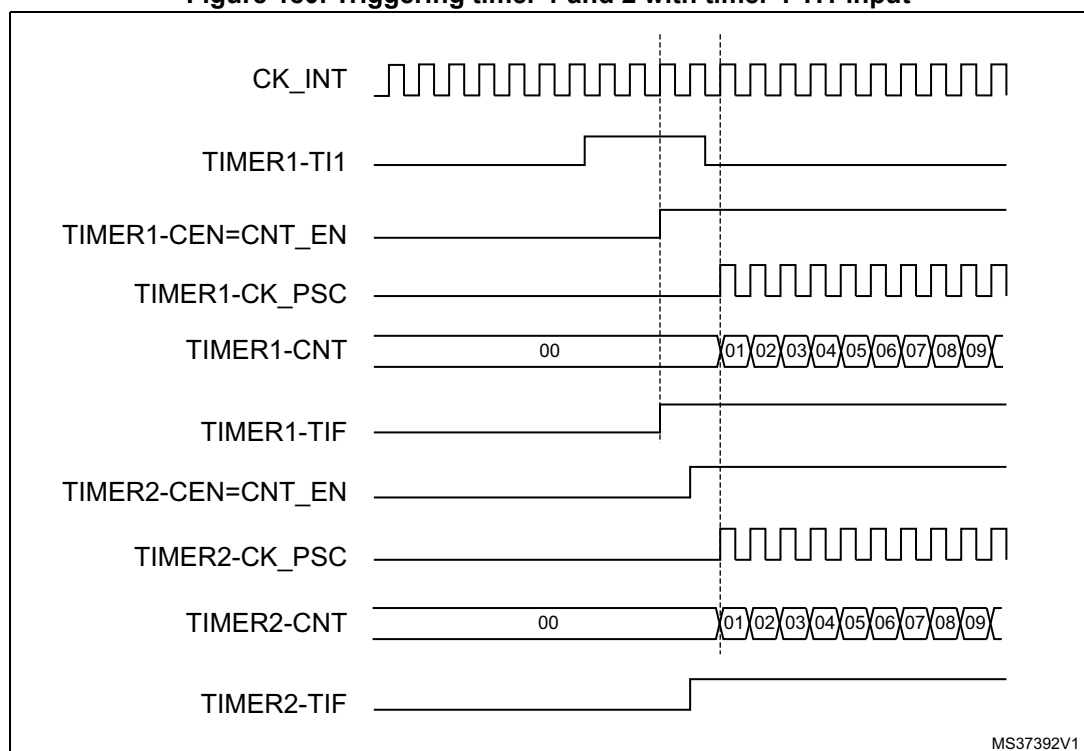
Figure 180. Triggering timer 1 and 2 with timer 1 TI1 input
