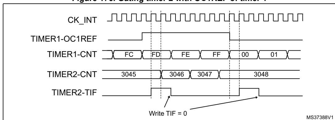
Figure 176. Gating timer 2 with OC1REF of timer 1
