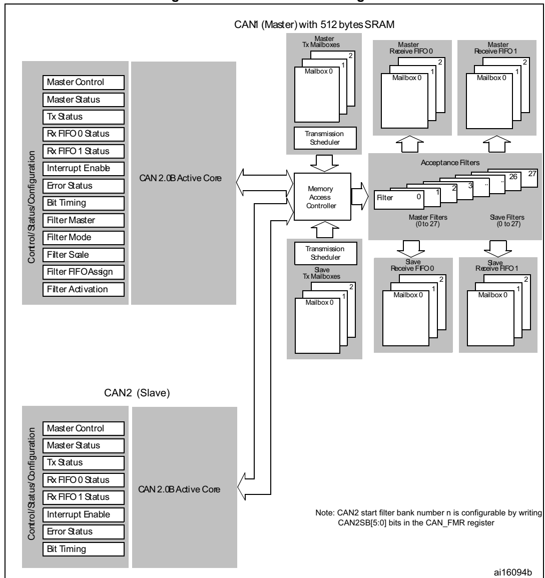
Figure 367. Dual CAN block diagram
