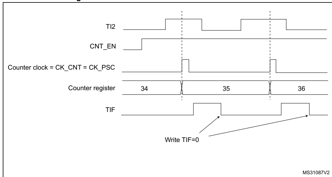
Figure 157. Control circuit in external clock mode 1
