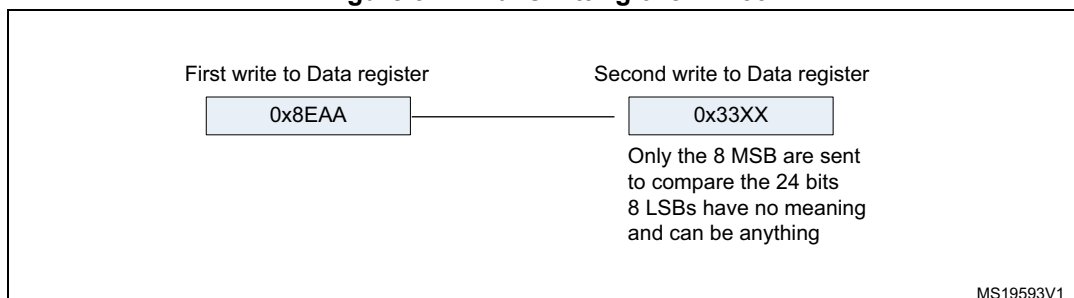
Figure 322. Transmitting 0x8EAA33
