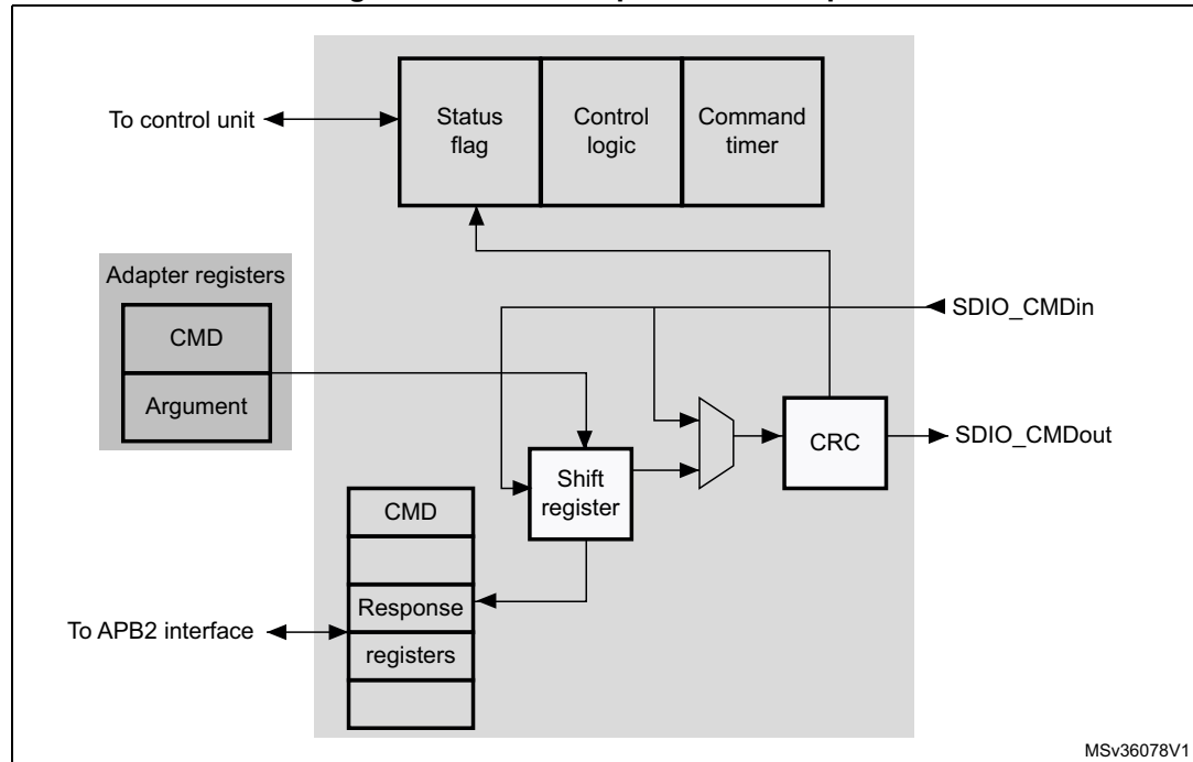
Figure 361. SDIO adapter command path
