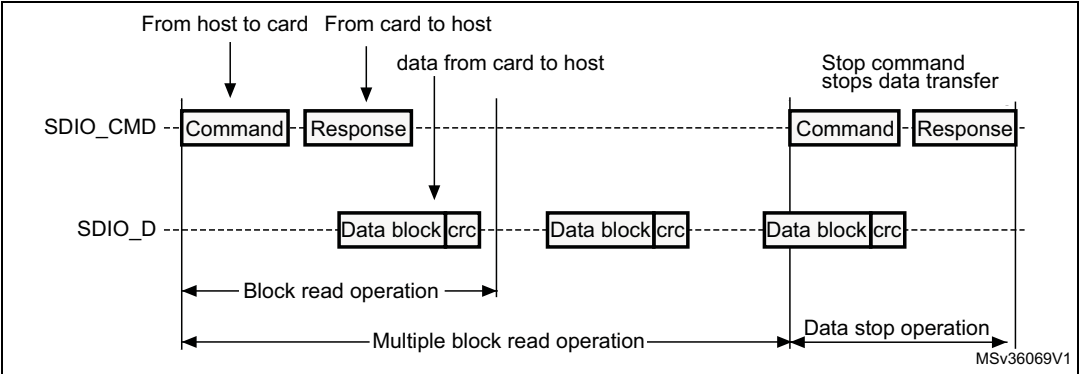
Figure 353. (Multiple) block read operation
