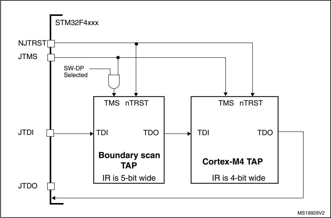
Figure 409. JTAG TAP connections
