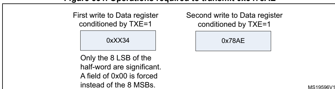
Figure 331. Operations required to transmit 0x3478AE
