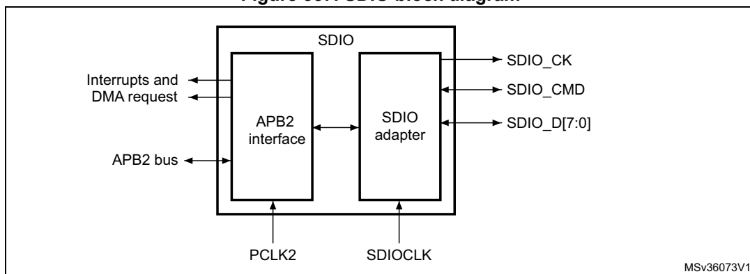
Figure 357. SDIO block diagram
