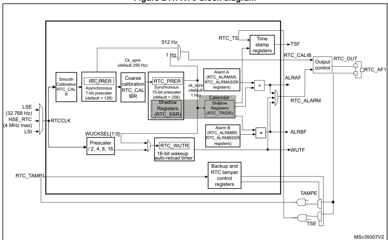
Figure 241. RTC block diagram
