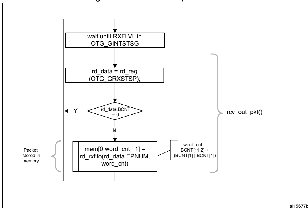
Figure 399. Receive FIFO packet read
