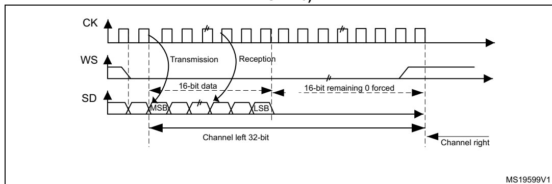
Figure 324. I 2 S Philips standard (16-bit extended to 32-bit packet frame with CPOL = 0)
