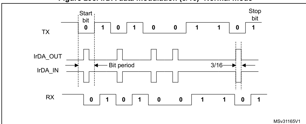
Figure 298. IrDA data modulation (3/16) -Normal mode
