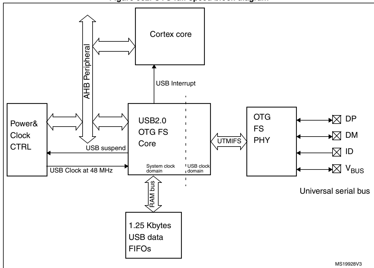
Figure 382. OTG full-speed block diagram
