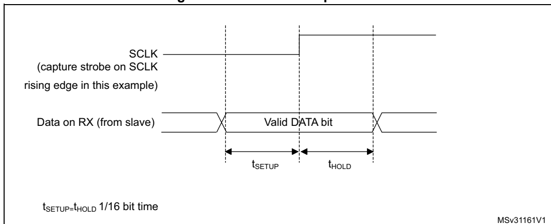
Figure 294. RX data setup/hold time
