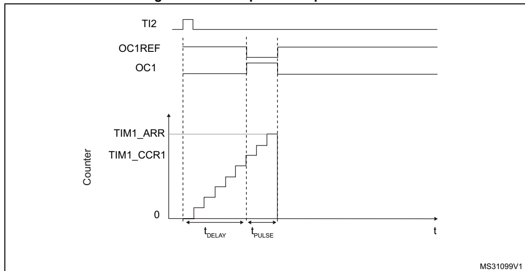
Figure 200. Example of one pulse mode.
