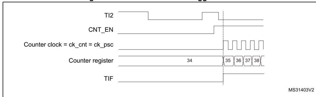
Figure 133. Control circuit in trigger mode
