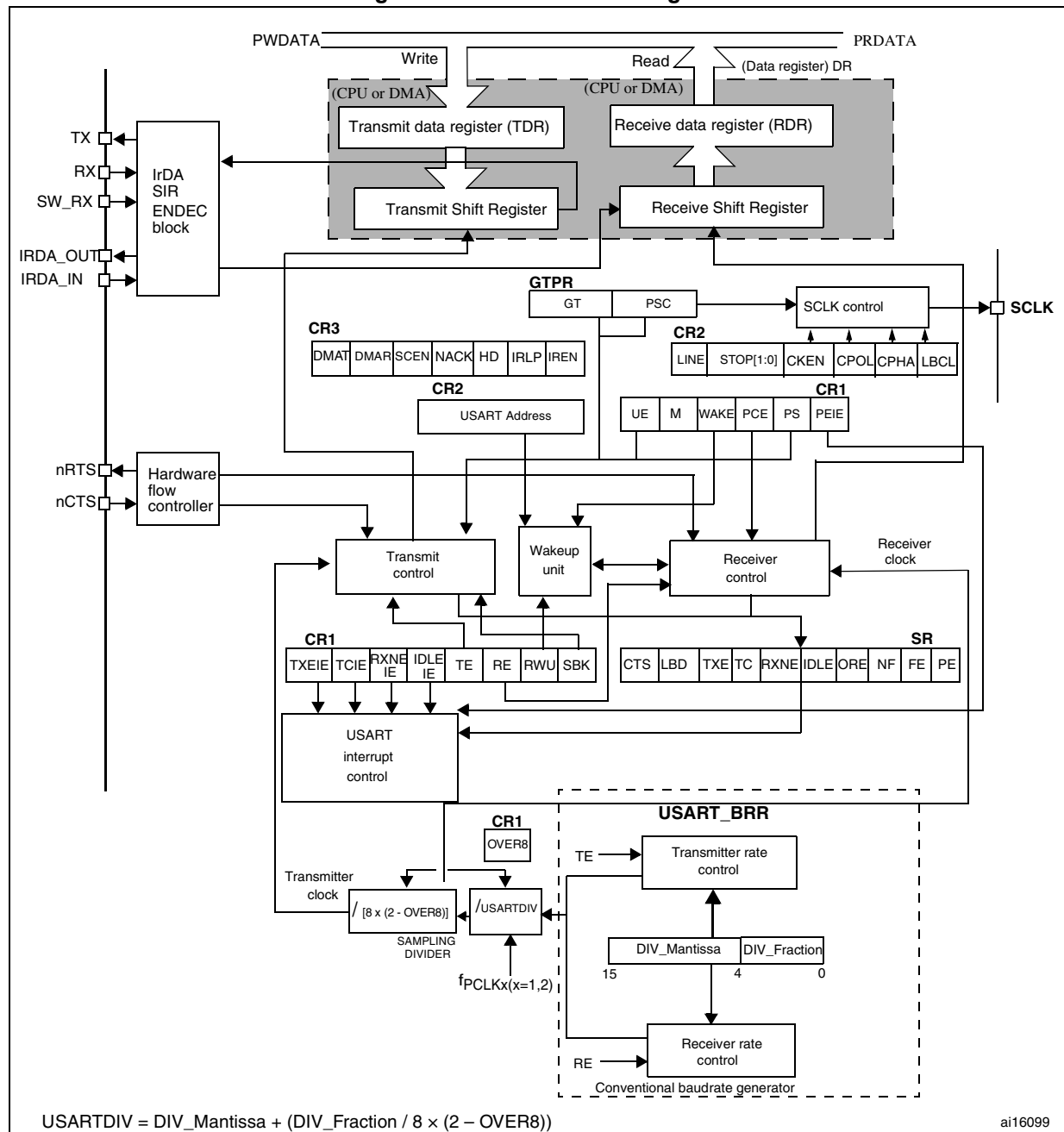
Figure 280. USART block diagram
