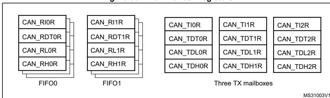
Figure 381. Can mailbox registers
