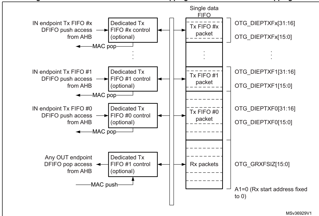
Figure 388. Device-mode FIFO address mapping and AHB FIFO access mapping
