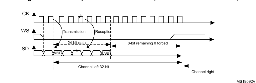
Figure 321. I 2 S Philips standard waveforms (24-bit frame with CPOL = 0)
