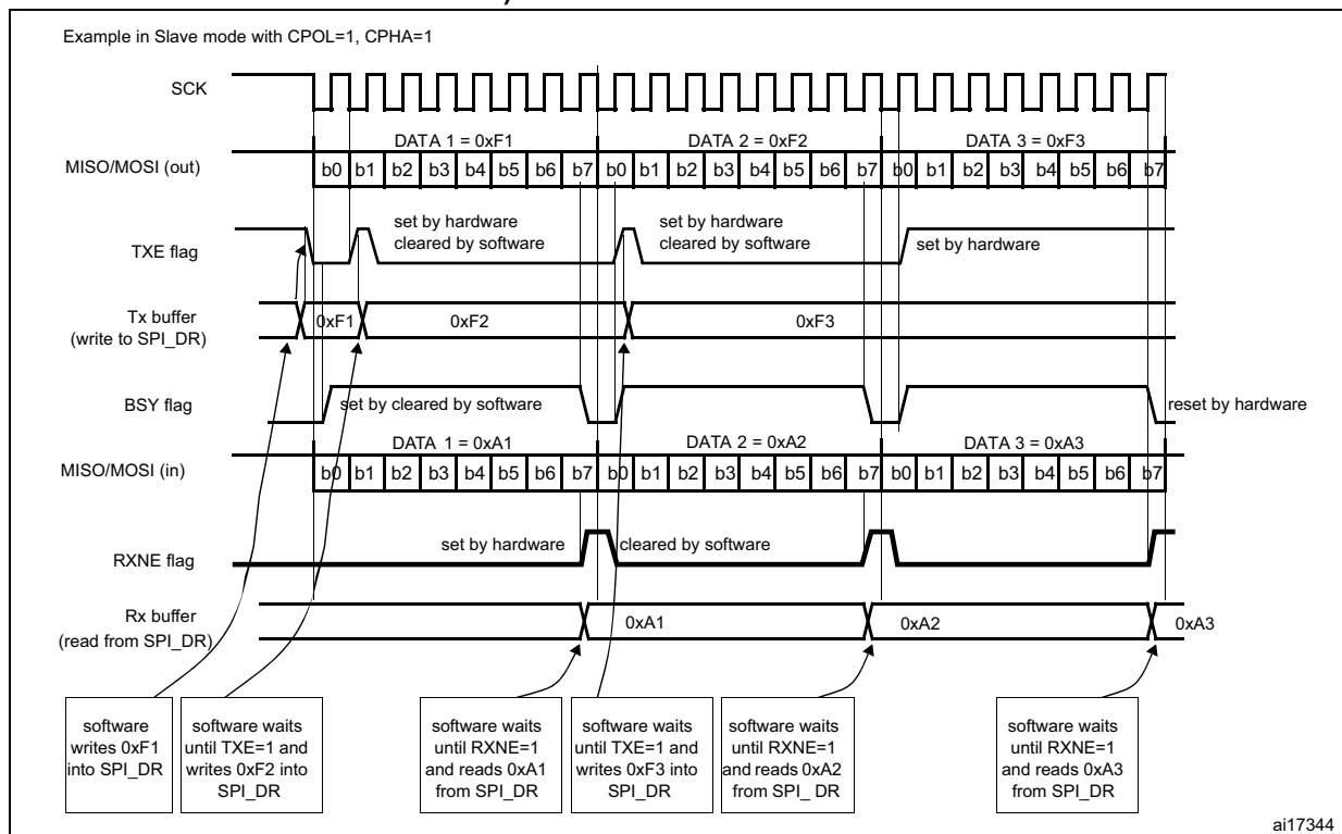
Figure 314. TXE/RXNE/BSY behavior in slave / full-duplex mode (BIDIMODE=0, RXONLY=0) in the case of continuous transfers
