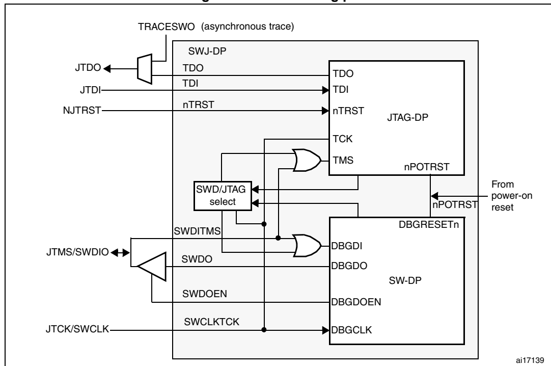
Figure 408. SWJ debug port
