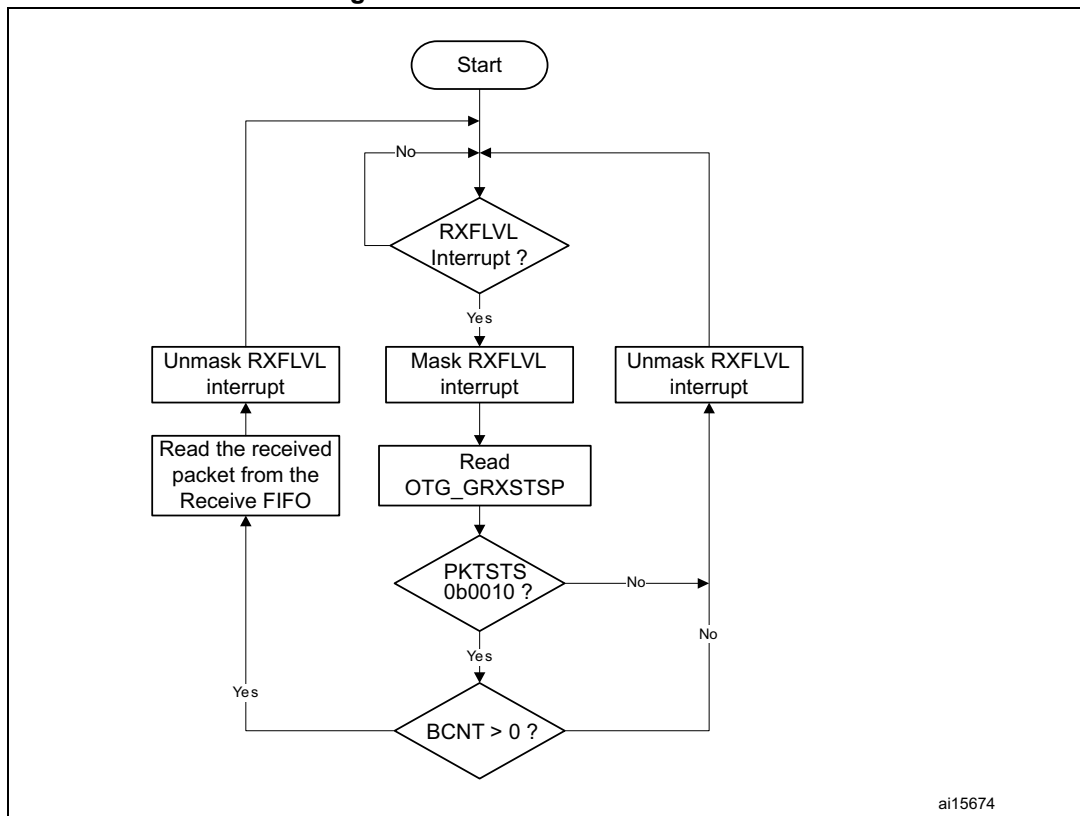
Figure 392. Receive FIFO read task
