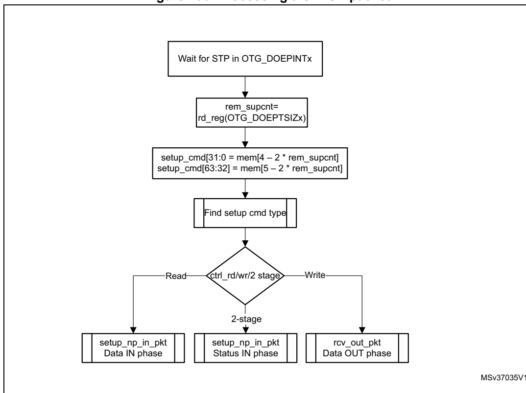
Figure 400. Processing a SETUP packet
