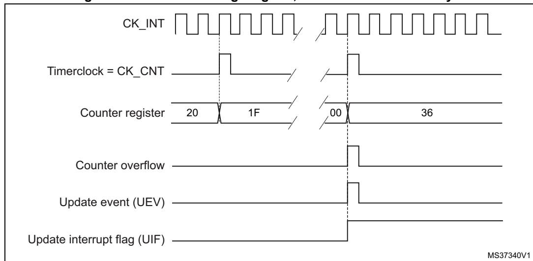
Figure 148. Counter timing diagram, Update event
