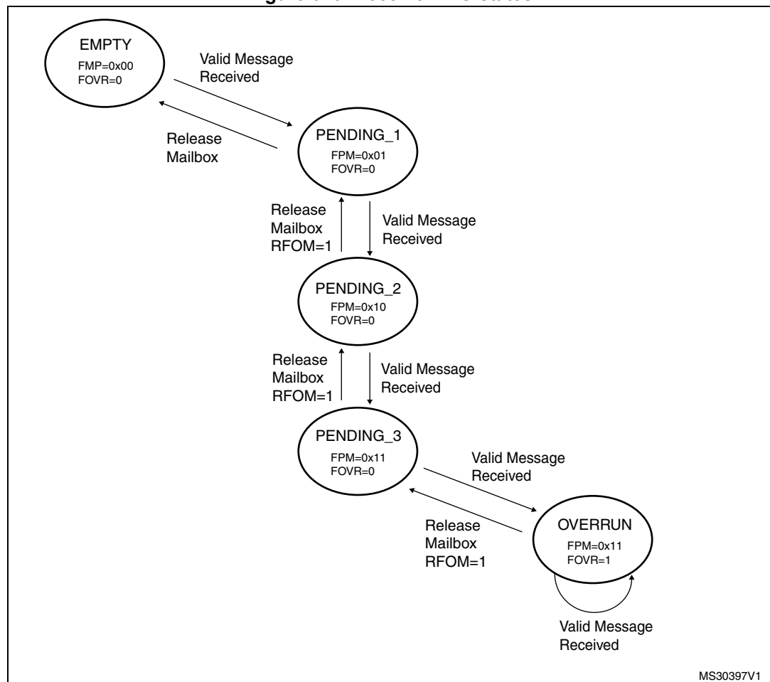
Figure 373. Receive FIFO states
