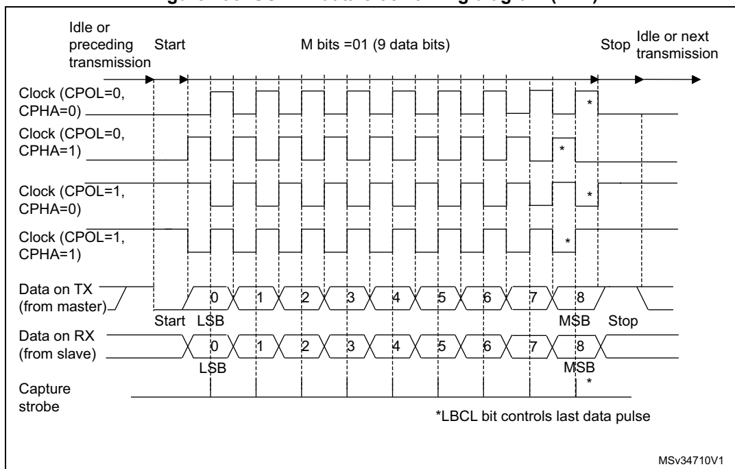
Figure 293. USART data clock timing diagram (M=1)
