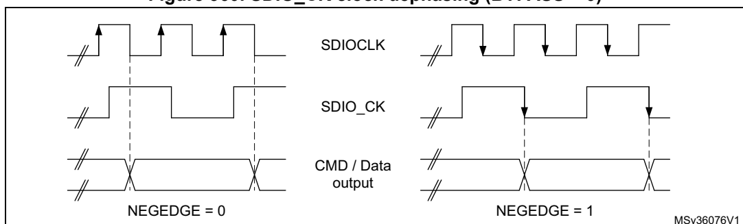
Figure 360. SDIO_CK clock dephasing (BYPASS = 0)
