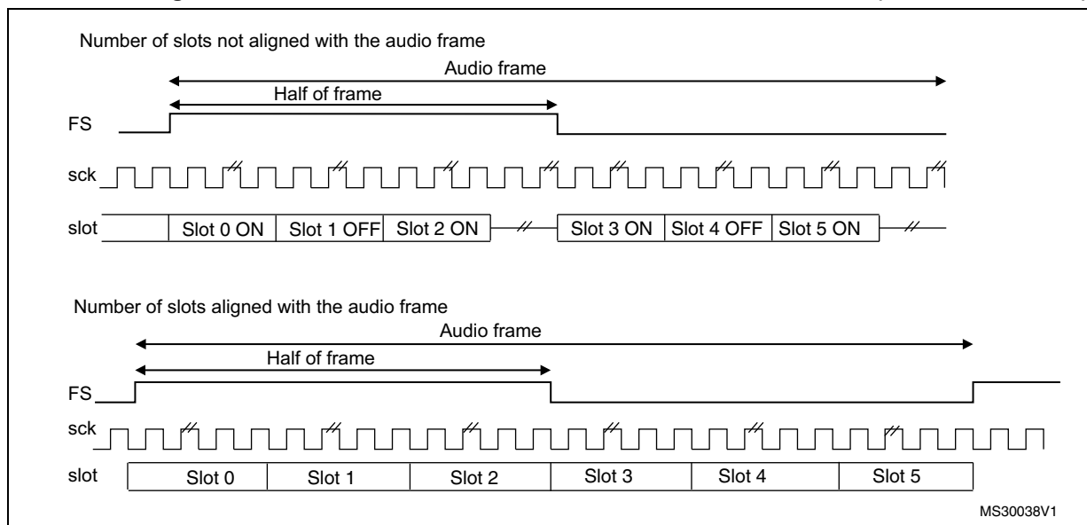
Figure 341. FS role is start of frame + channel side identification (FSDEF = TRIS = 1)
