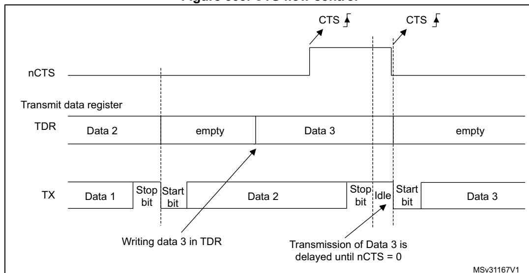
Figure 303. CTS flow control
