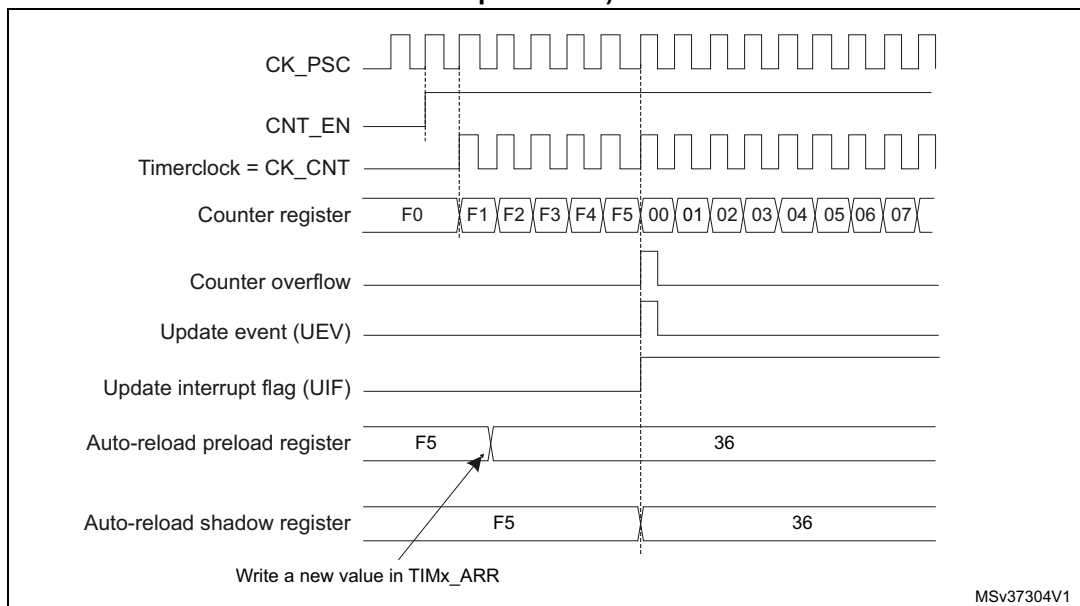
Figure 143. Counter timing diagram, Update event when ARPE=1 (TIMx_ARR preloaded)
