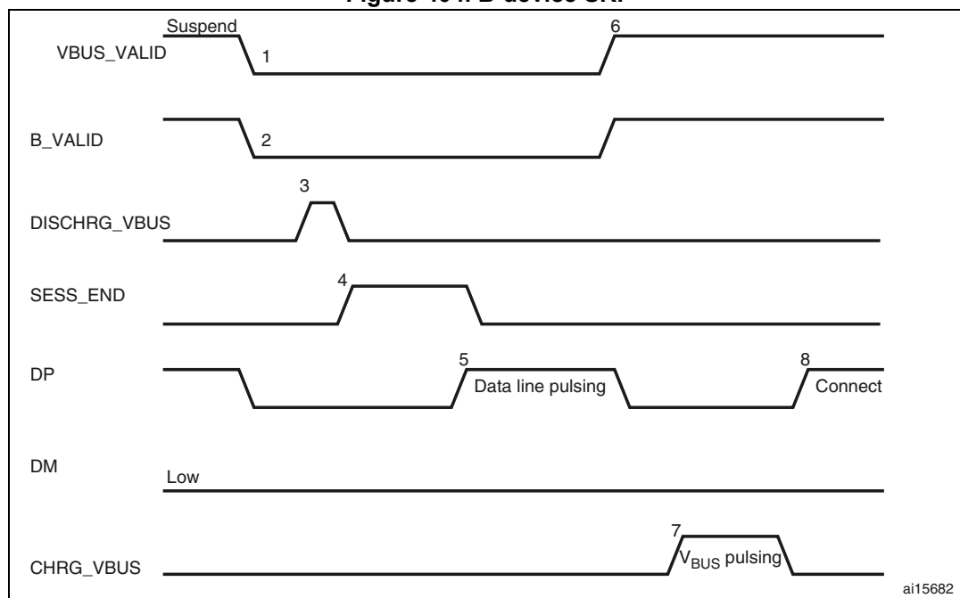
Figure 404. B-device SRP
