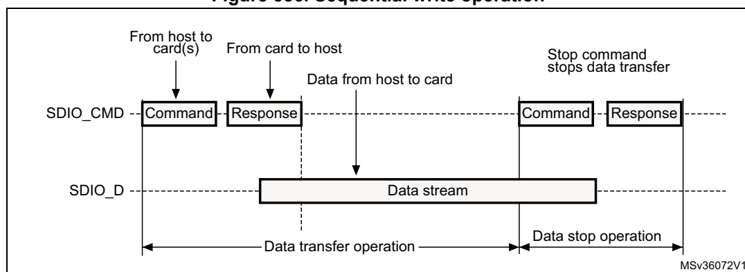
Figure 356. Sequential write operation
