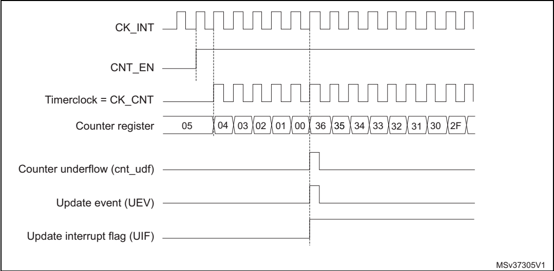
Figure 144. Counter timing diagram, internal clock divided by 1
