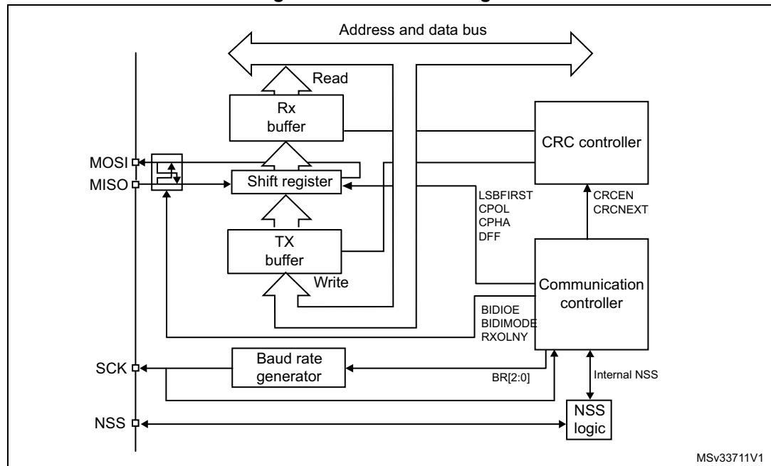
Figure 305. SPI block diagram
