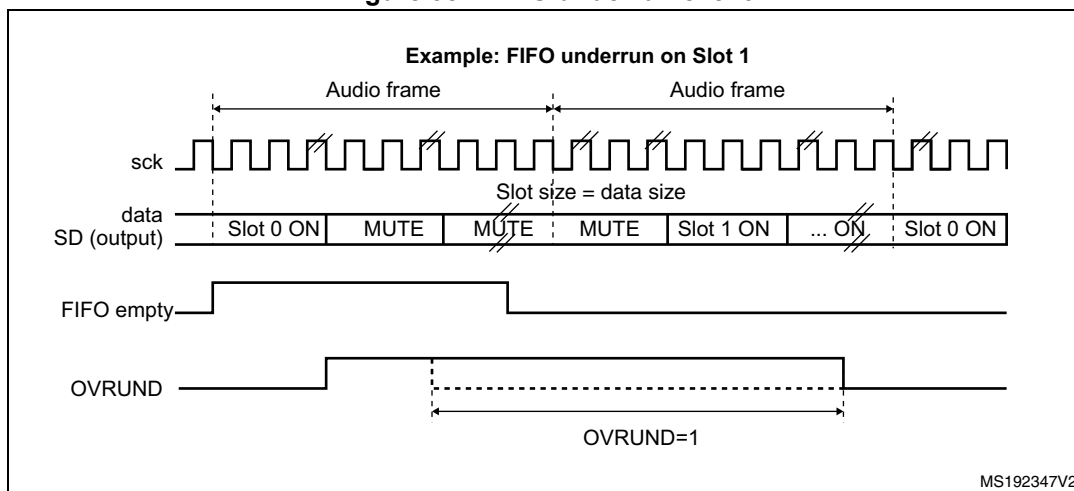
Figure 351. FIFO underrun event
