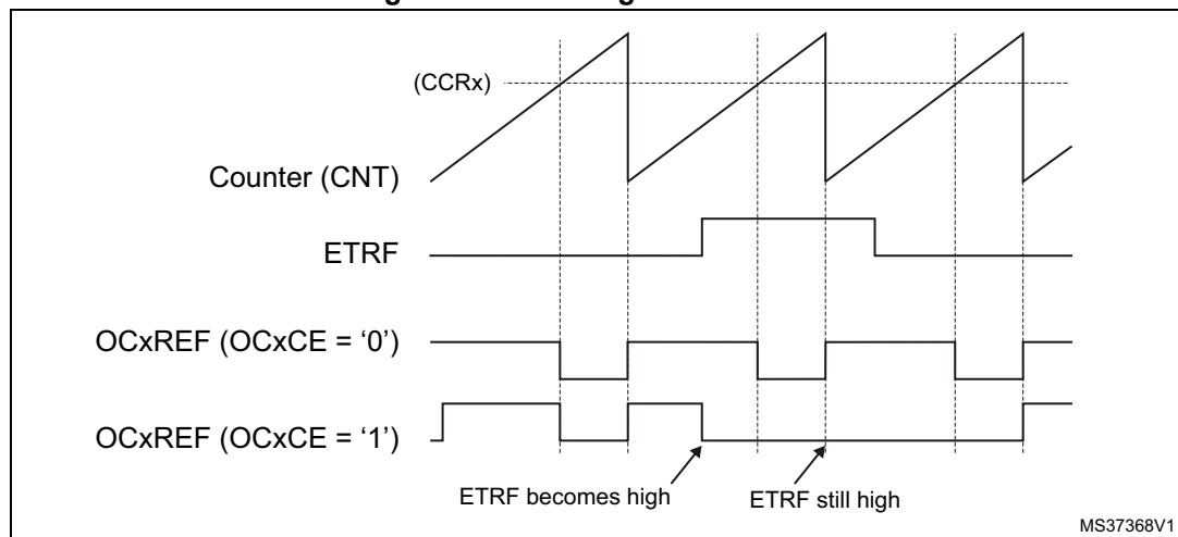
Figure 168. Clearing TIMx OCxREF
