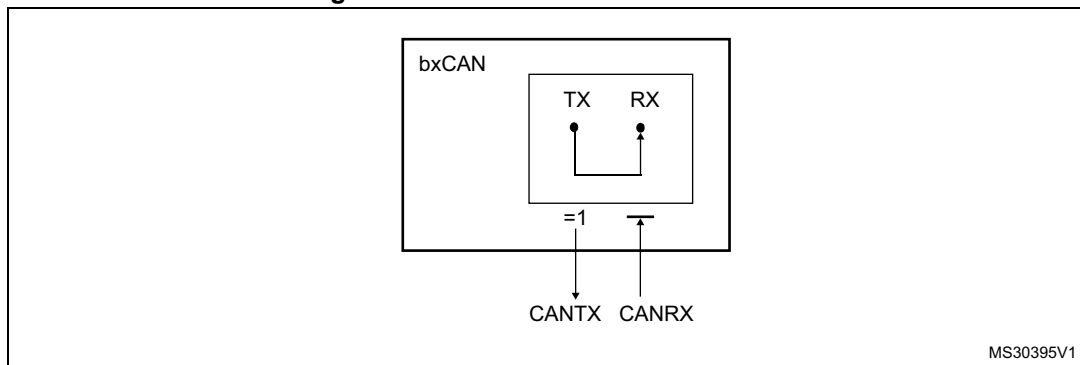
Figure 371. bxCAN in combined mode
