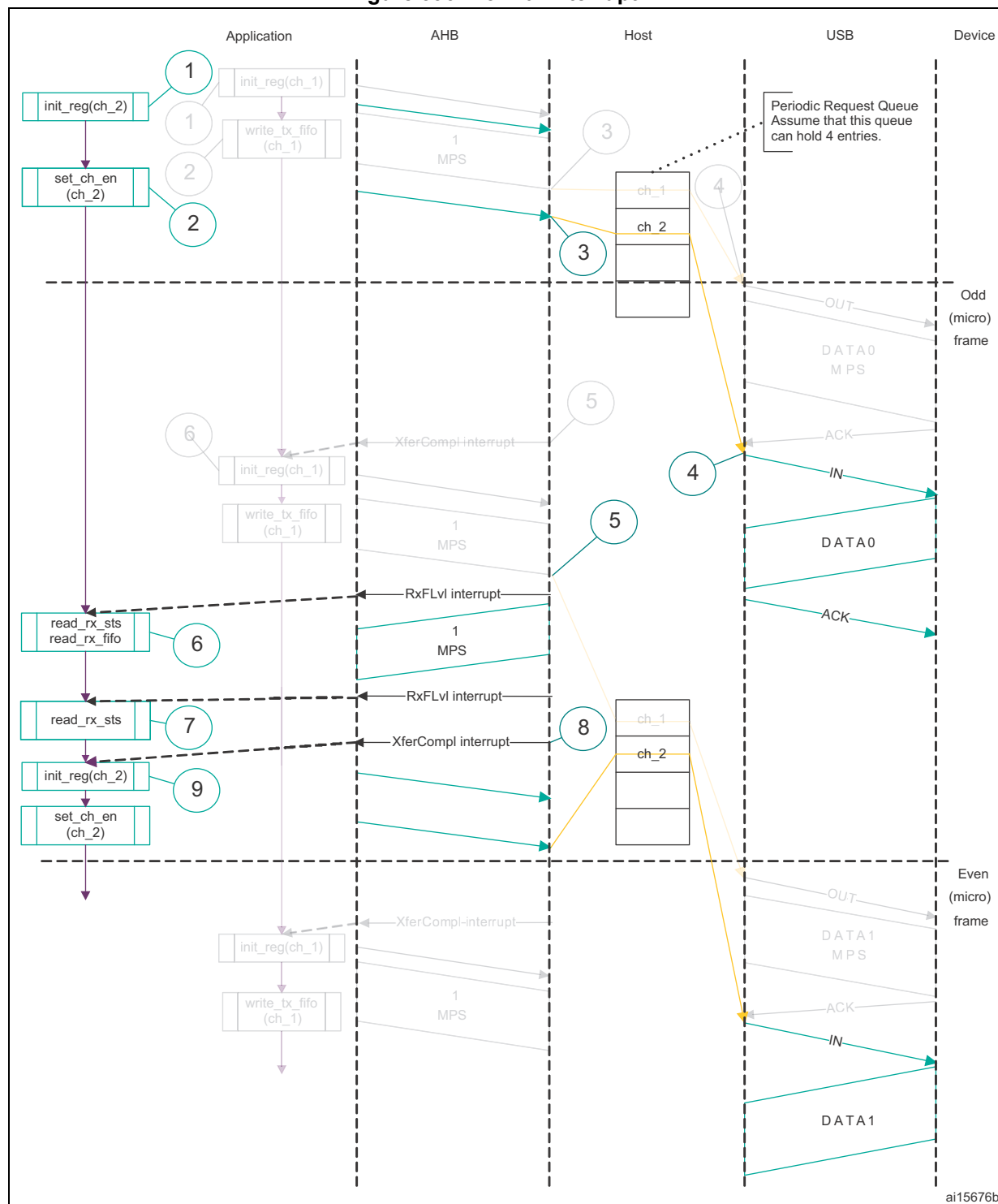
Figure 396. Normal interrupt IN
