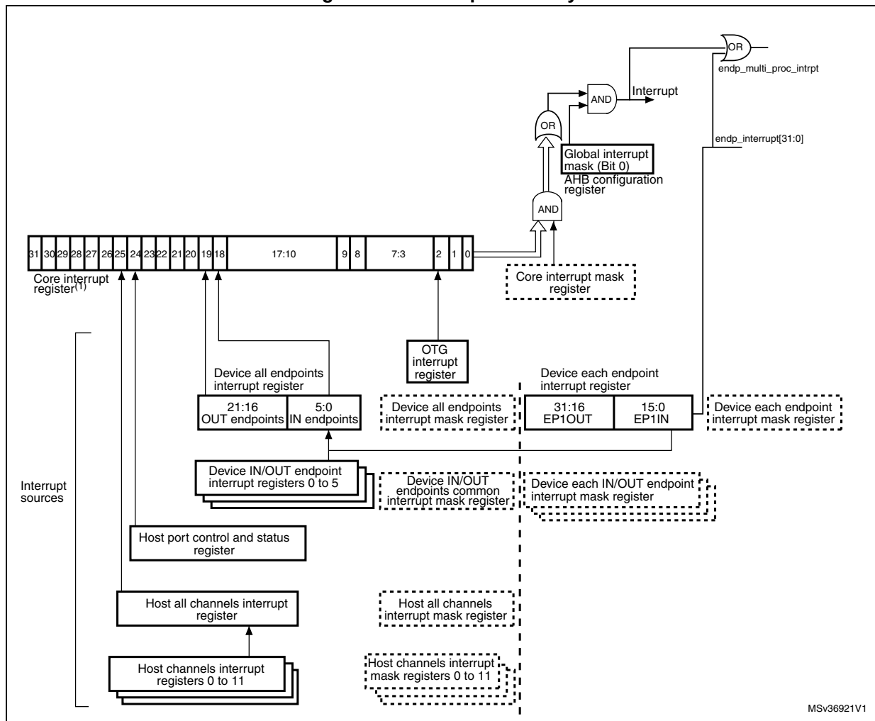
Figure 390. Interrupt hierarchy
