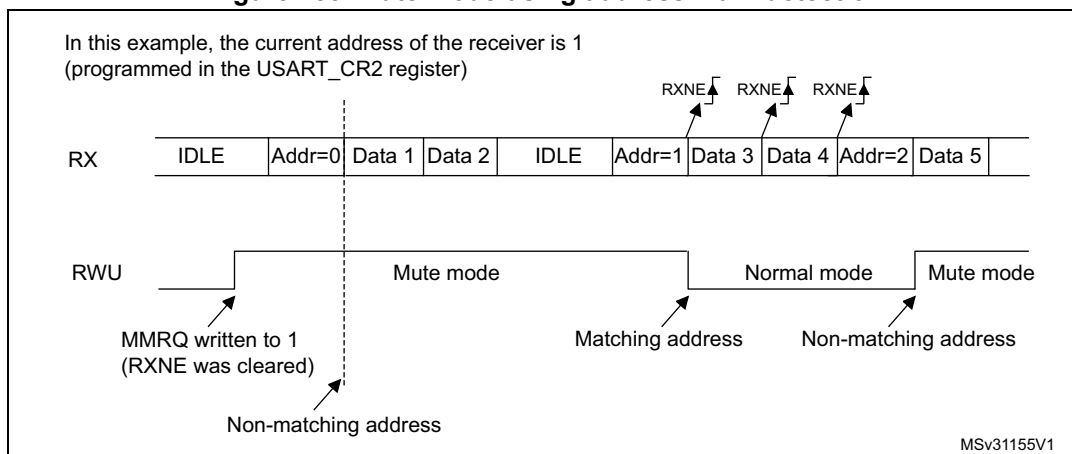
Figure 288. Mute mode using address mark detection
