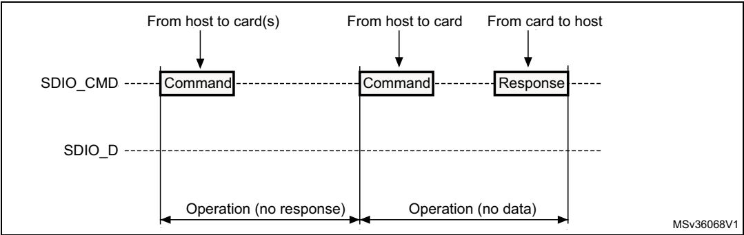
Figure 352. “No response” and “no data” operations
