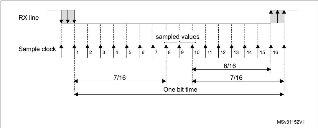
Figure 285. Data sampling when oversampling by 16
