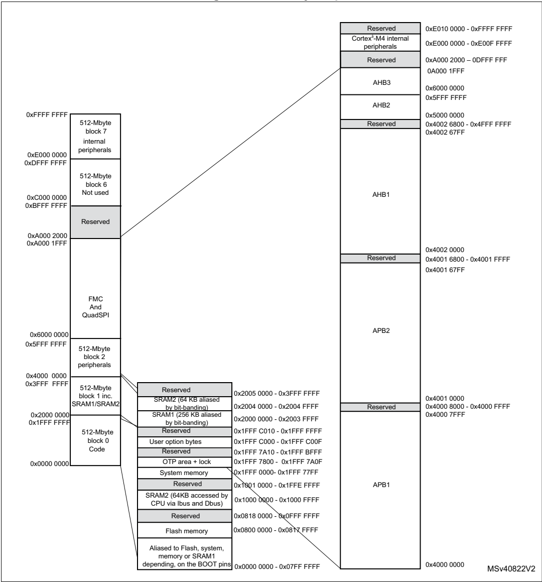
Figure 2. Memory map
