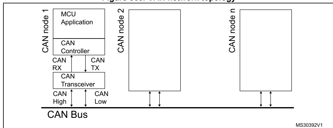
Figure 366. CAN network topology
