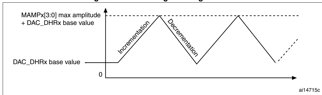
Figure 73. DAC triangle wave generation
