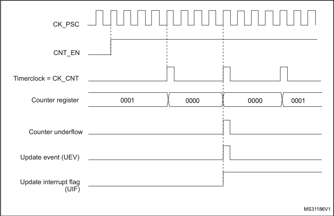
Figure 98. Counter timing diagram, internal clock divided by 4
