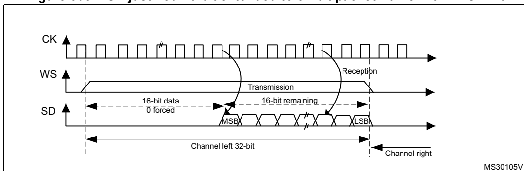
Figure 333. LSB justified 16-bit extended to 32-bit packet frame with CPOL = 0
