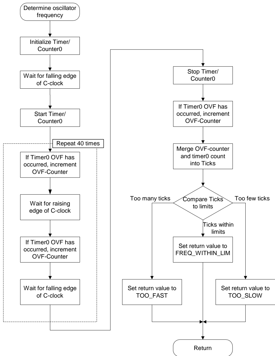
Figure 3. Flowchart of algorithm determining relationship between the C-clock and the internal oscillator frequency.
